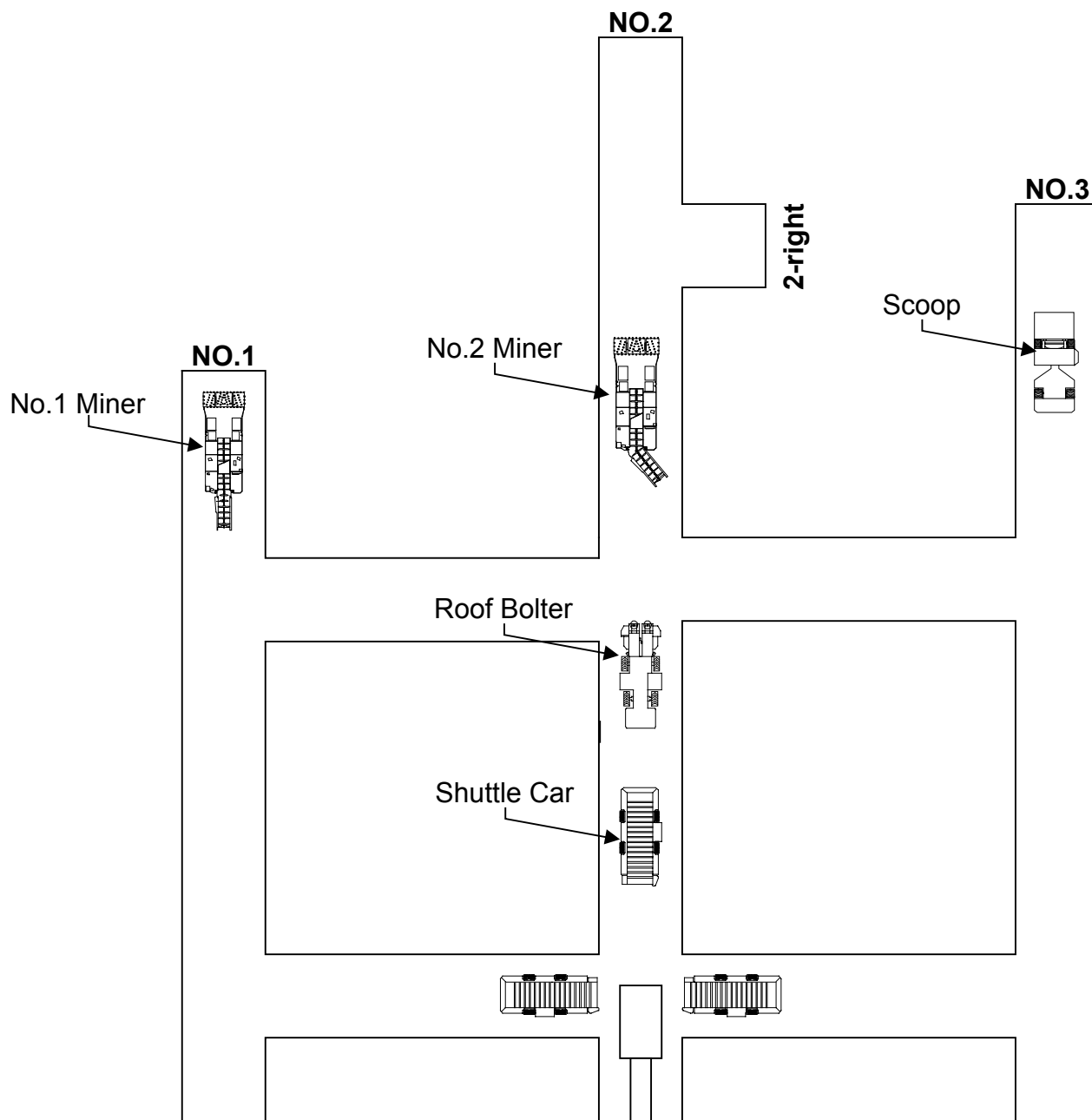
Figure 1 - No.2 Miner parked in entry after completing cut in 2-right crosscut. Roof bolter waiting to pull into 2-right to begin installing roof supports.
