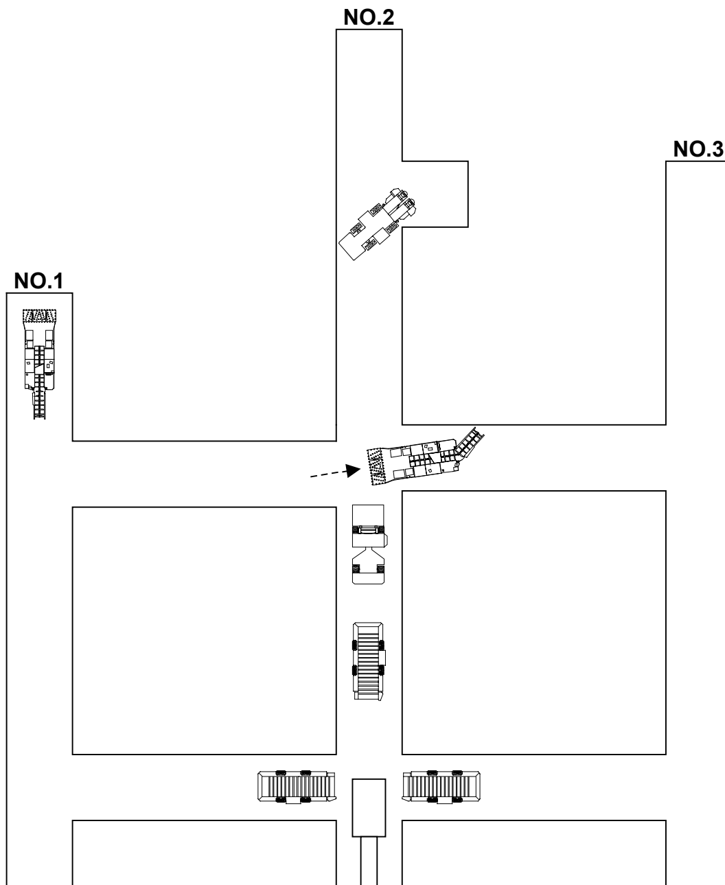
Figure 4 - No.2 miner moved back across intersection to allow scoop to proceed inby in the No.2 entry. The accident occurred during this move.
