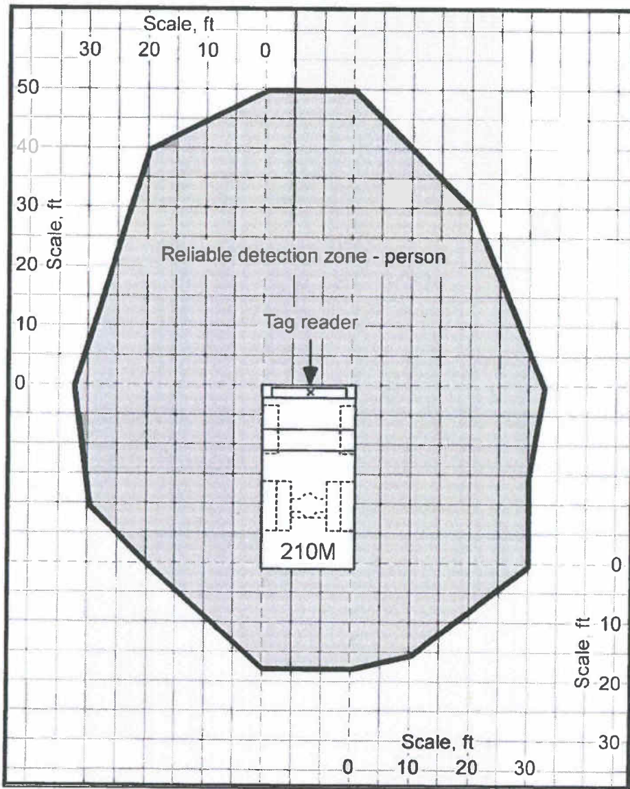
Figure 27. Buddy system detection zone for a person wearing a tag.
