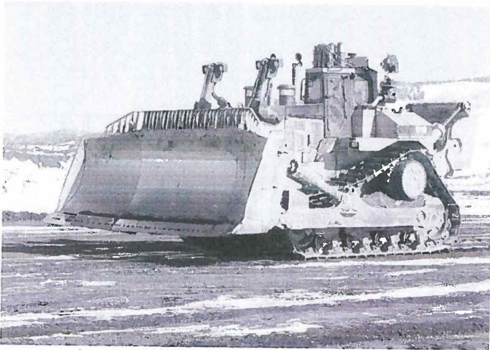
Figure A.10. Caterpillar D11R dozer.
