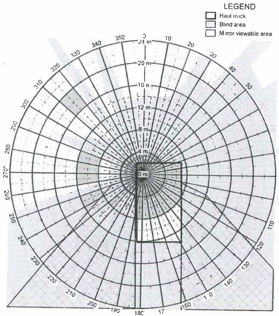
Figure A.2. Blind area diagram for a Euclid EH4500 280-ton-capacity haul truck (ground plane).
