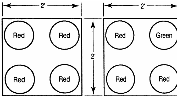
Figure 12.-Determination of surface brightness by averaging method.
