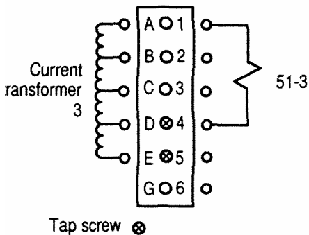
Figure 31.- Terminals A and D are connected to the relay coils. However, since D and E are shorted and they are both terminals of the current transformer secondaries, the current transformers are effectively shorted. Any two or more terminals of a current transformer that are shorted will short out the entire secondary. Also, the current transformer secondaries are not properly grounded.
