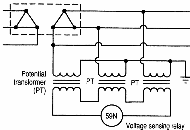
Figure 25.-Grounded-phase protection scheme for ungrounded systems.
