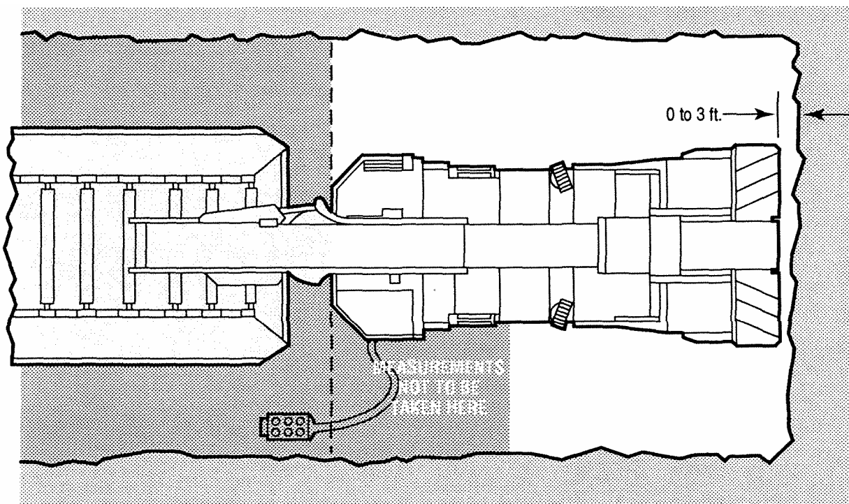
Figure 8.-Surface from which light measurements may be taken when remotely controlled continuous mining machines are operated in working places where the mining height is less than 42 inches. Measurements shall not be taken of the floor area between the cutter boom hinge pin or gathering head hinge pin and the coal face.
