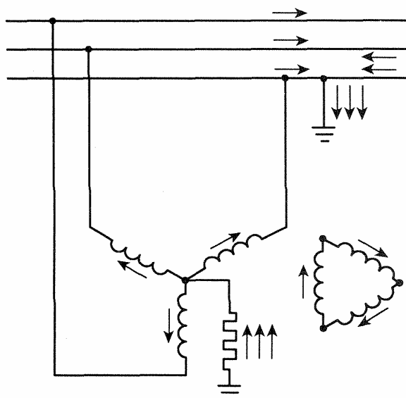
Figure 18.—Connections and current distribution in a wye-delta grounding transformer.
