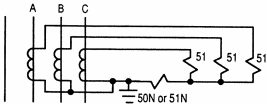
Figure 23.-Residual trip relaying to provide grounded-phase protection.
