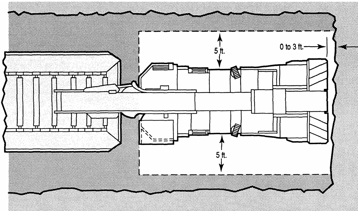
Figure 7.-Surfaces from which light measurements may be taken when the mining height is less than 42 inches.
