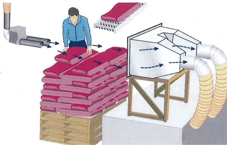
Figure 4-14. Semiautomated pallet loading system using push-pull ventilation.
