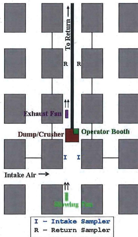
Figure 2-4. Sampling locations used to isolate dust generated at an underground crusher.
