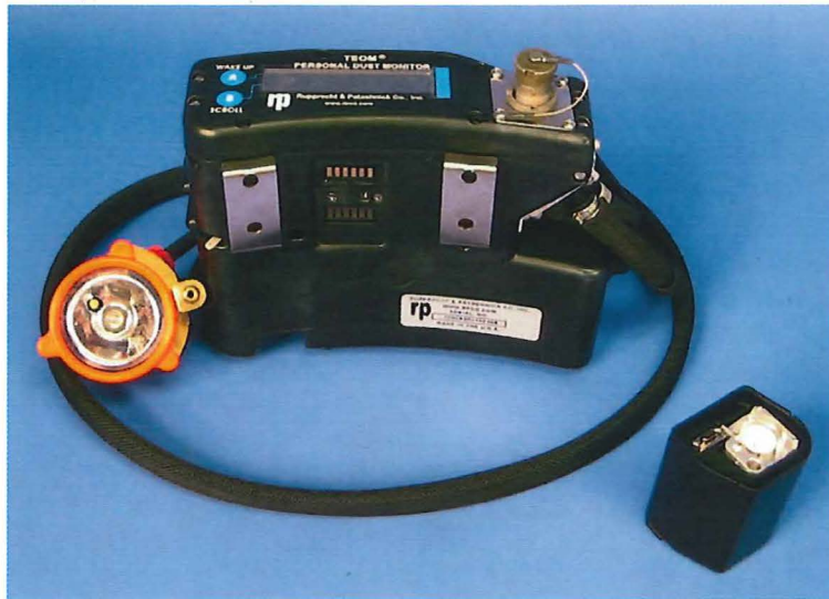
Figure 2-3. Personal dust monitor (PDM) with TEOM unit removed and shown on right.
