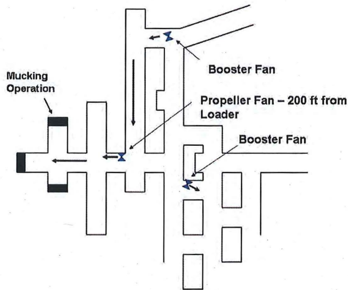
Figure 3-7. Fans positioned to ventilate dead-end entries.
