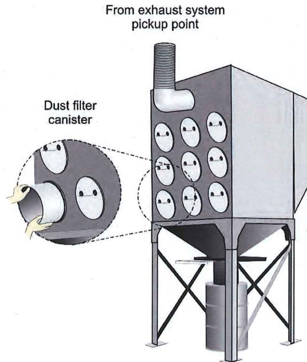
Figure 4-7. Canister-type dust collector system.
