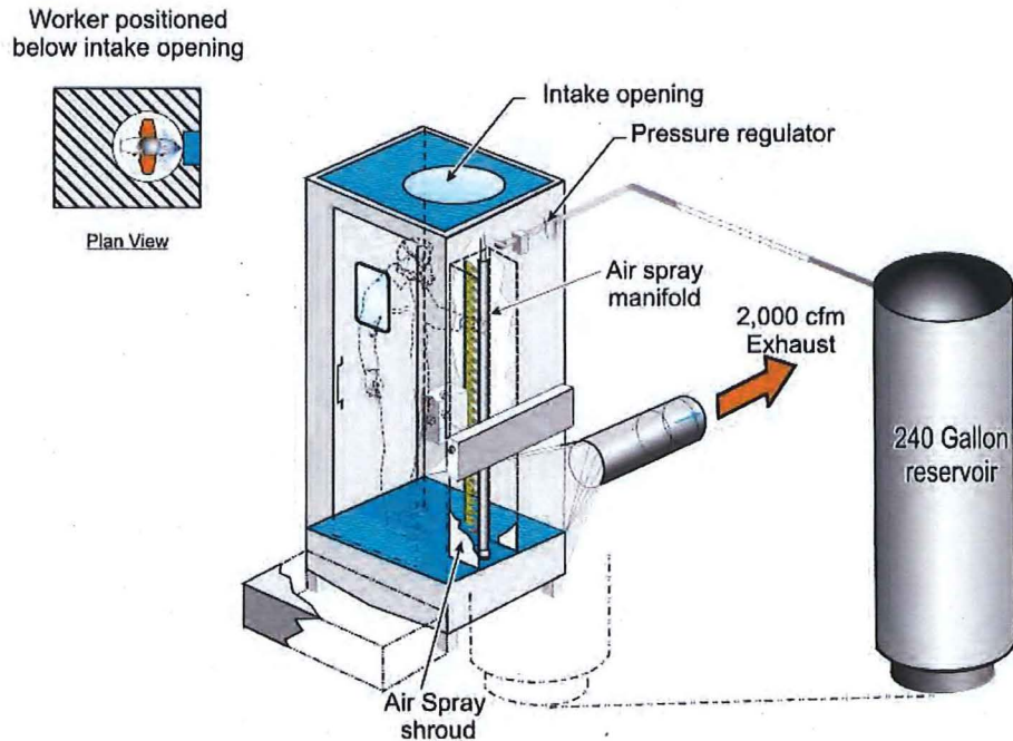
Figure 4-16. Clothes cleaning system design.
