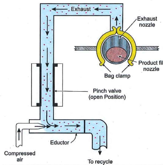
Figure 4-12. Dual bag nozzle design.
