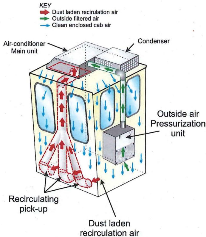
Figure 3-3. Filtration and pressurization system components and design.
