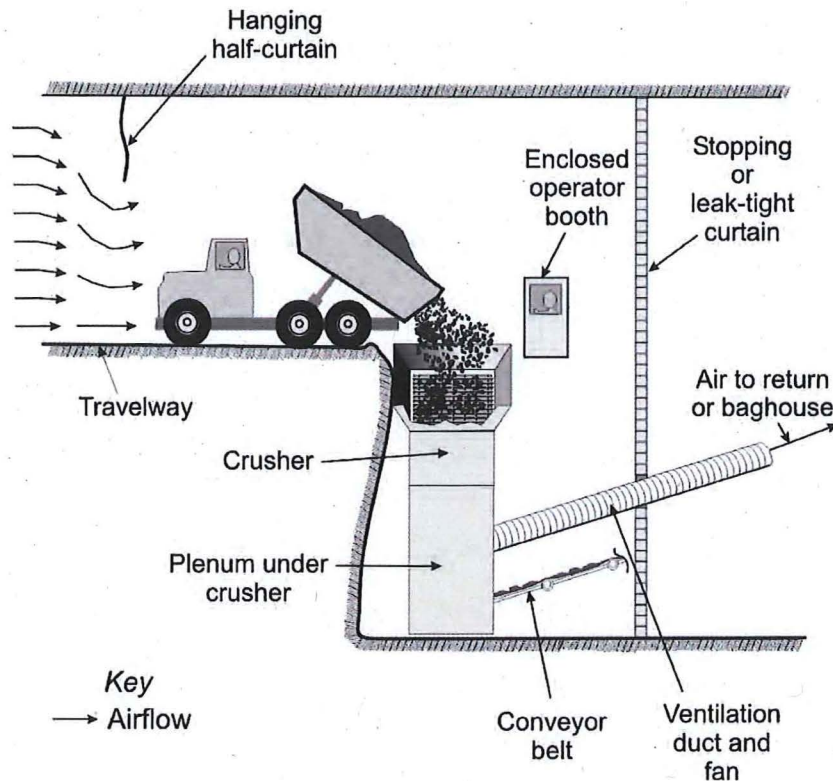
Figure 3-2. Closed ventilation system using plenum.
