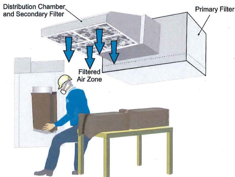
Figure 4-19 - Overhead air supply island system.
