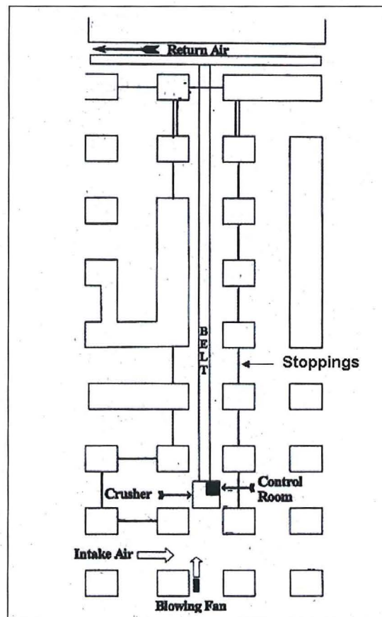
Figure 3-1. Typical method used to isolate crushing facility from mine air.
