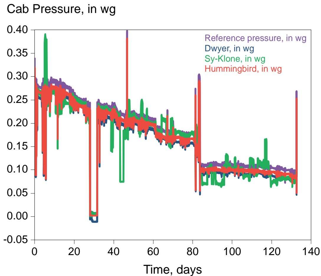
Figure 10.17. Graphical comparison of pressure readings from three units under a field test and one reference gauge during an in-mine test.
