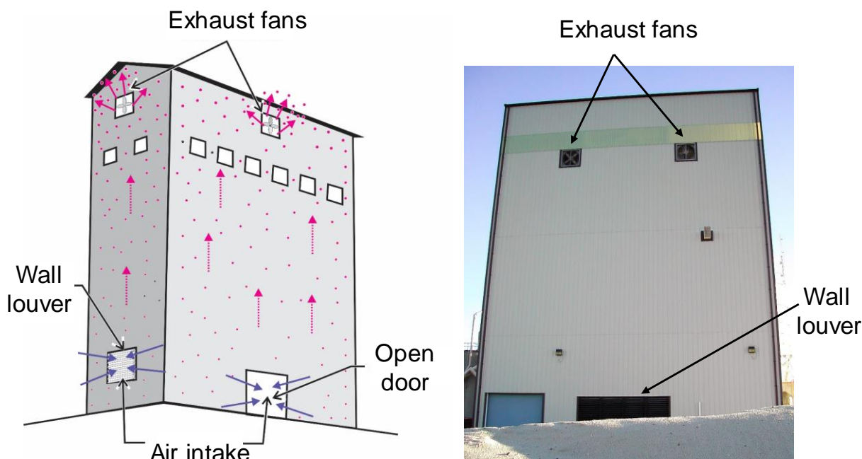
Figure 9.11. Illustration and photo showing the basic design of a total structure ventilation system.
