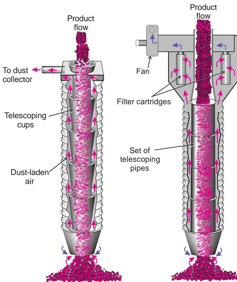
Figure 8.1. Illustration of loading spouts designed with telescoping cups or pipes and dust collection capabilities.
