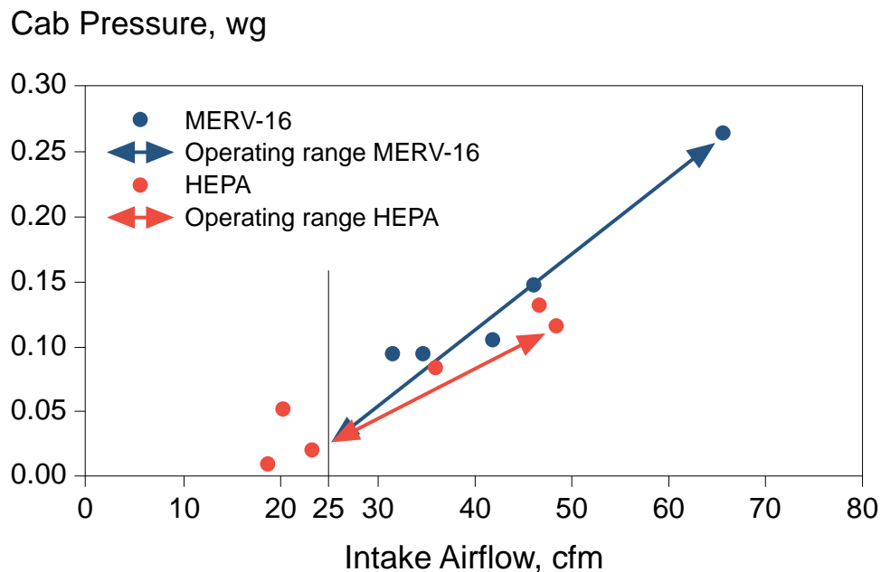
Figure 10.14. Graphical comparison of the intake airflows and positive cab pressures for a face drill test at a mine site comparing MERV-16 and HEPA filters.
