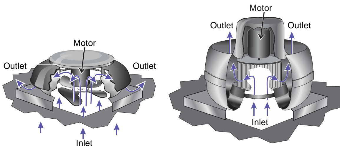
Figure 2.33. Illustration of typical roof ventilators using axial fans (left) and centrifugal fans (right).
