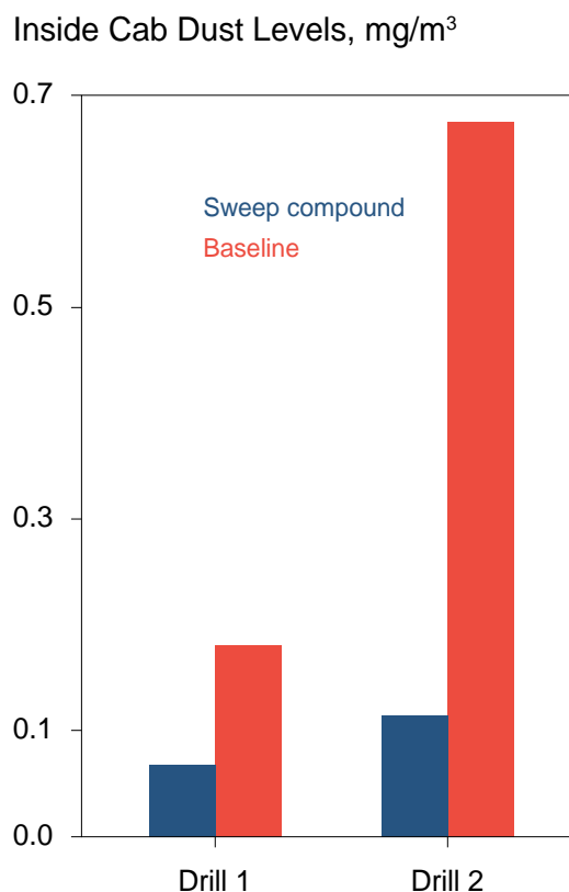
Figure 9.26. Bar chart showing respirable dust concentrations inside the enclosed cabs of two different pieces of equipment with and without the use of a gritless nonpetroleum-based sweeping compound.
