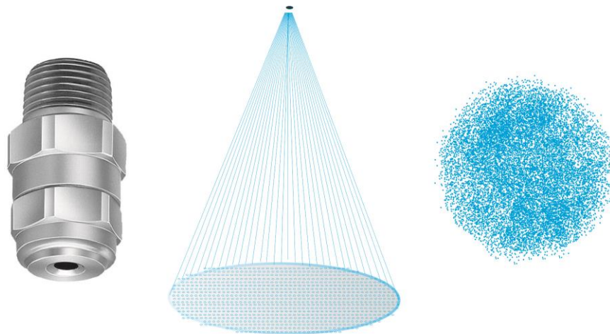
Figure 3.7. Typical full cone nozzle and spray pattern [adapted from Schick 2008].
