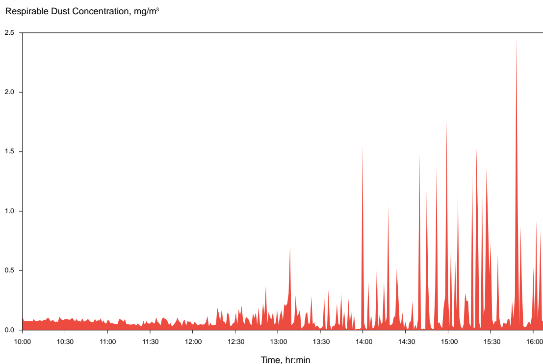
Figure 11.9. Graph showing respirable dust concentrations measured from a haul road after water application occurred at 10:00 at one operation [from Organiscak and Reed 2004].
