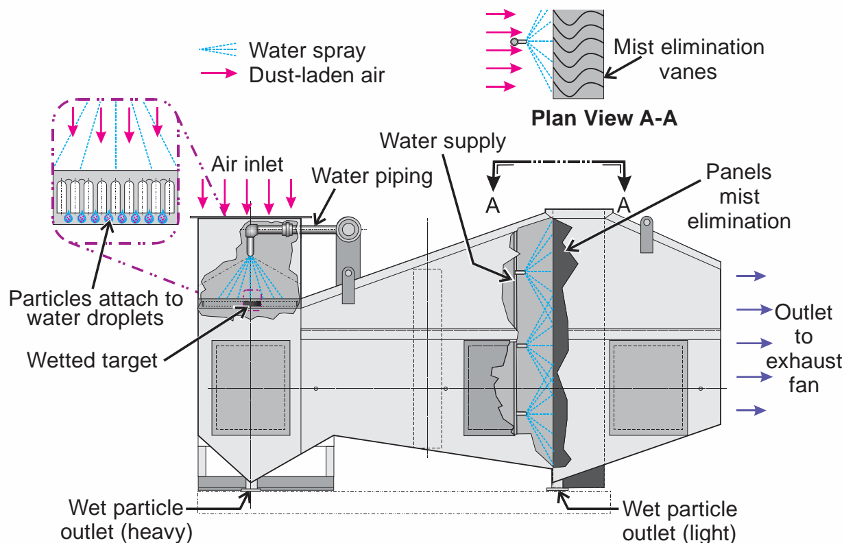
Figure 2.22. Illustration showing a typical design of a wet scrubber dust collector.
