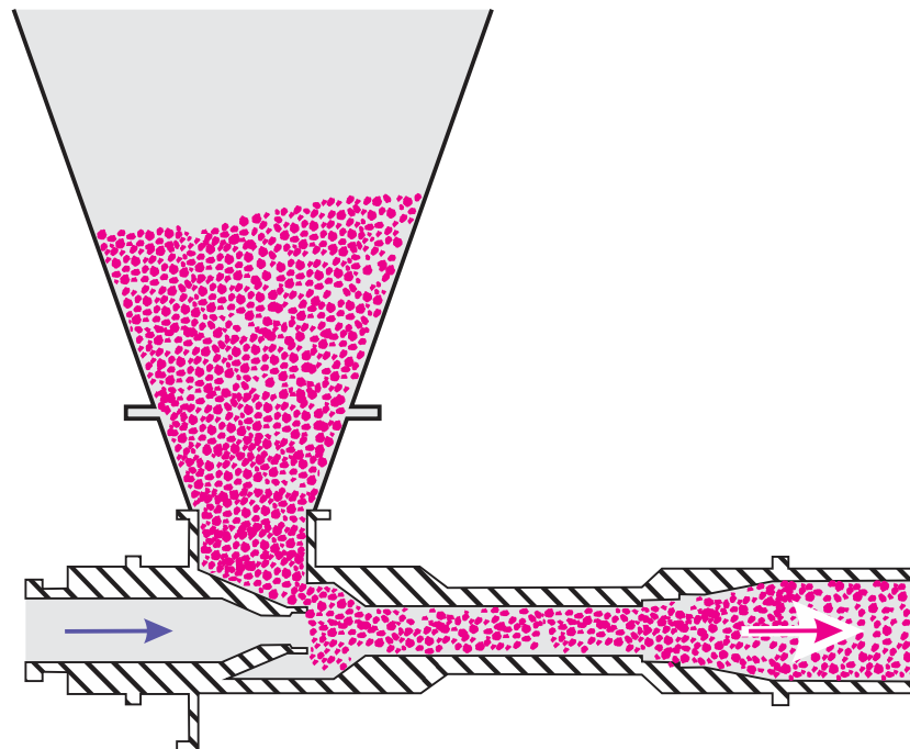
Figure 6.29. Illustration of a venturi eductor utilizing suction to draw the feed material into the conveying line.
