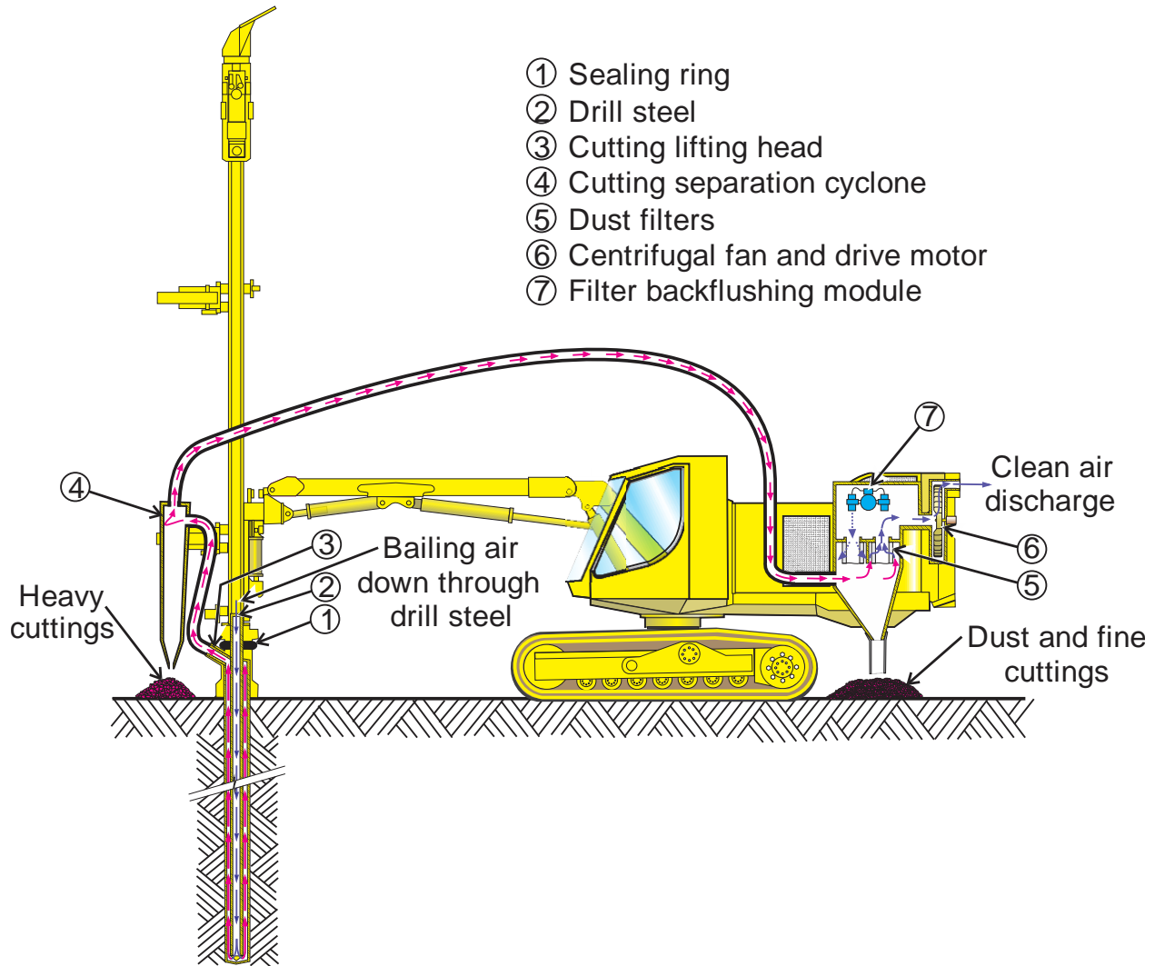
Figure 4.18. Illustration of a typical dust collector system used by small crawler (or “buggy”) drills.
