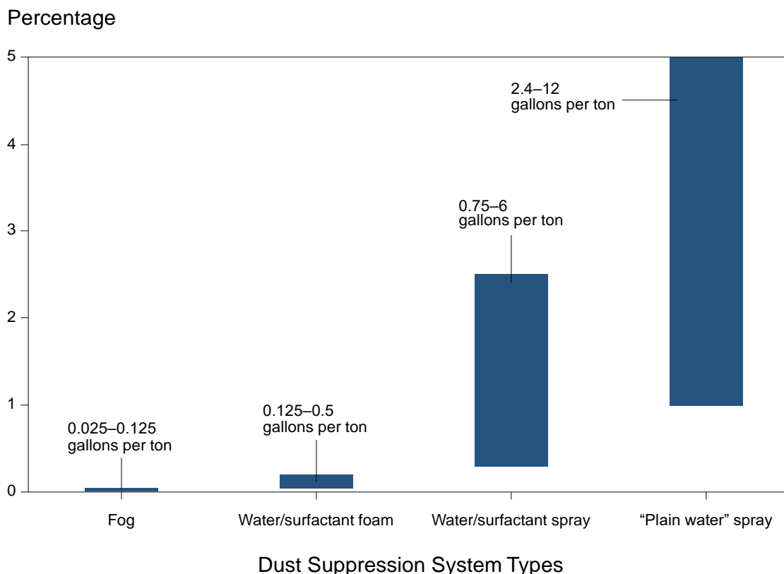
Figure 3.1. Typical rates of moisture addition for various dust suppression systems [adapted from Swinderman et al. 2009].
