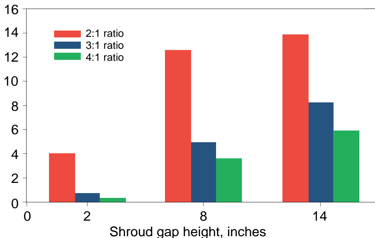
Figure 4.7. Results of changing the collector to bailing airflow ratio at various shroud gap heights.
