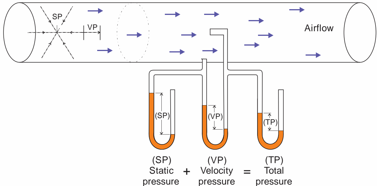
Figure 2.1. Illustration of the relationship between static pressure, velocity pressure, and total pressure [adapted from ACGIH 2010]. Example represents suction side of the fan.
