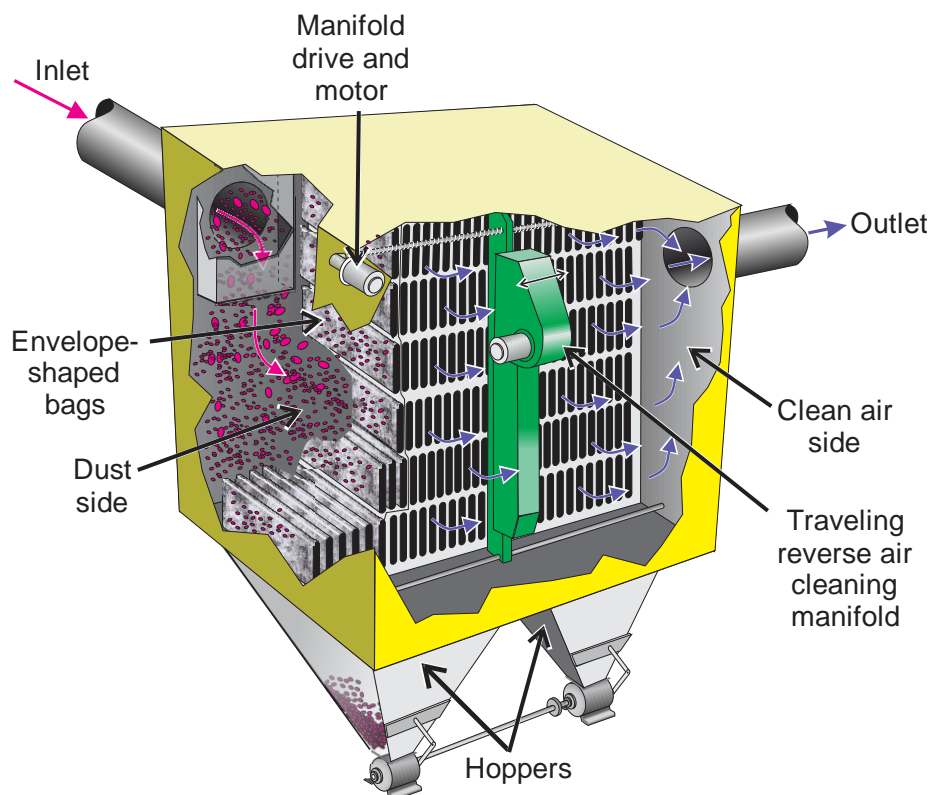
Figure 2.19. Illustration showing a typical design of a reverse air dust collector.
