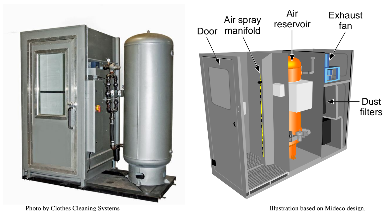
Figure 9.5. Two clothes cleaning systems using compressed air at 30 psig to remove dust from work clothing.
