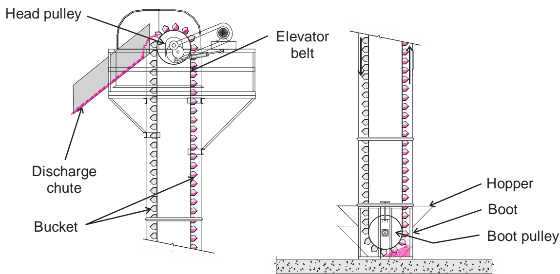
Figure 6.23. Illustration of a bucket elevator.
