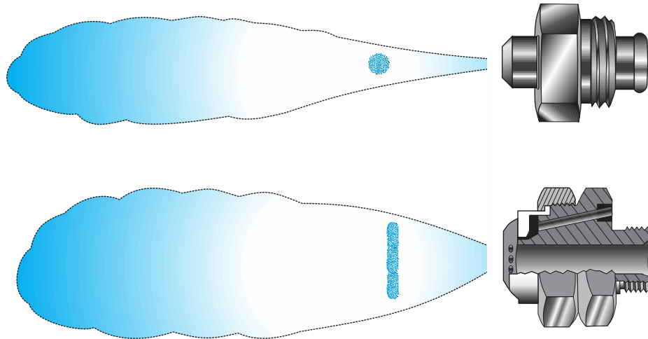
Figure 3.6. Two types of nozzle spray patterns. The top illustration shows a typical air atomizing nozzle round spray pattern. The bottom illustration shows a typical fan spray pattern [adapted from SSCO 2018].
