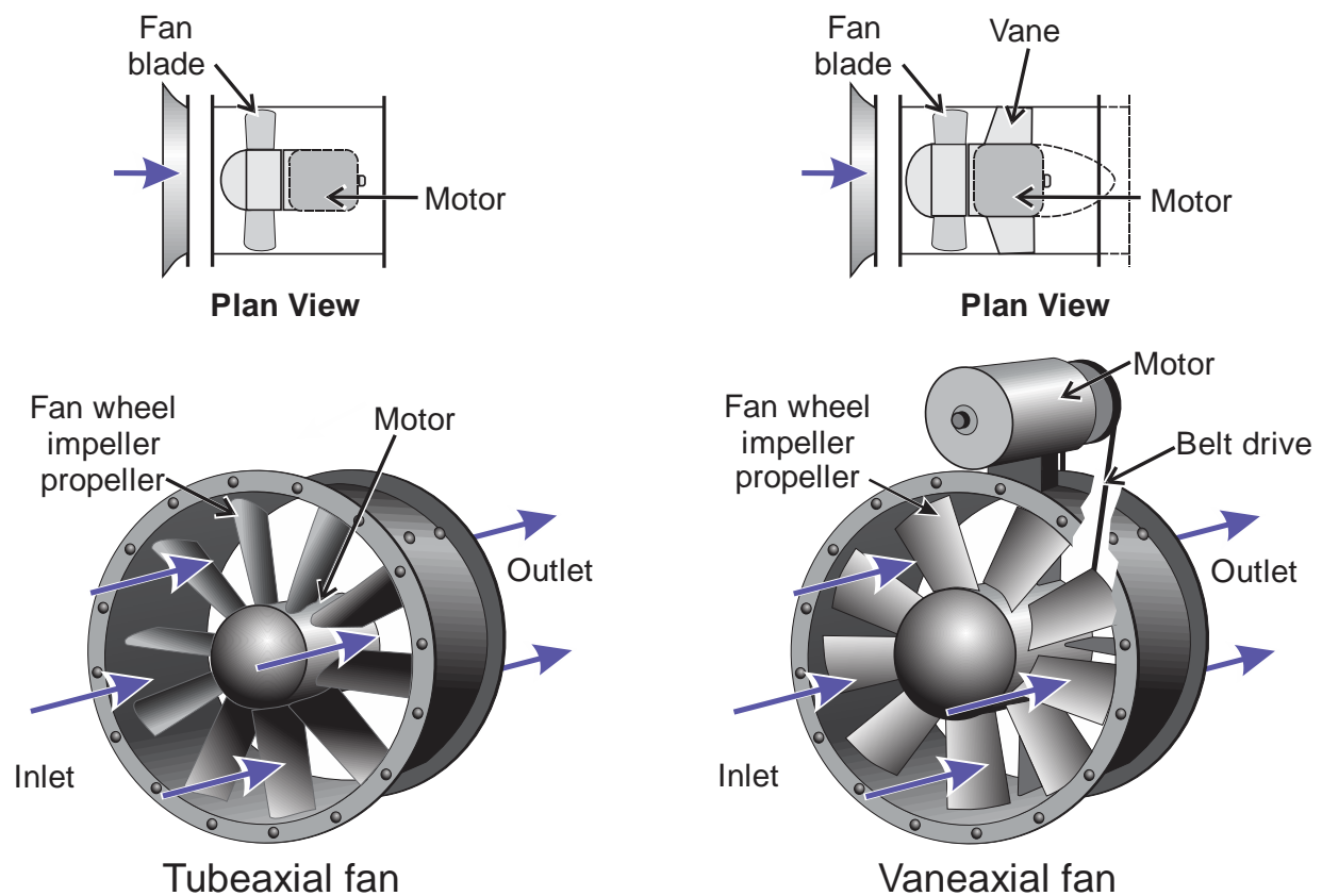
Figure 2.30. Illustration of a typical tubeaxial fan (left) and vaneaxial fan (right).
