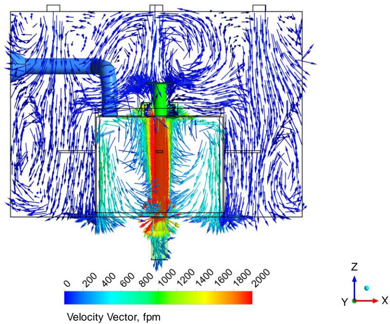
Figure 4.11. Velocity vectors for a cross-sectional plane (shroud without air-blocking shelves) with a detailed view underneath the table.
