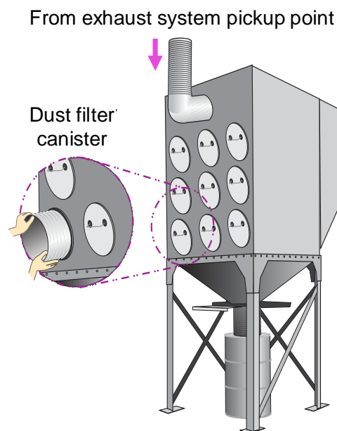
Figure 2.21. Cartridge collector with dust filter canisters. The left illustration shows a cutaway of a canister being replaced. The photo on the right shows a cartridge collector with the canisters mounted horizontally.
