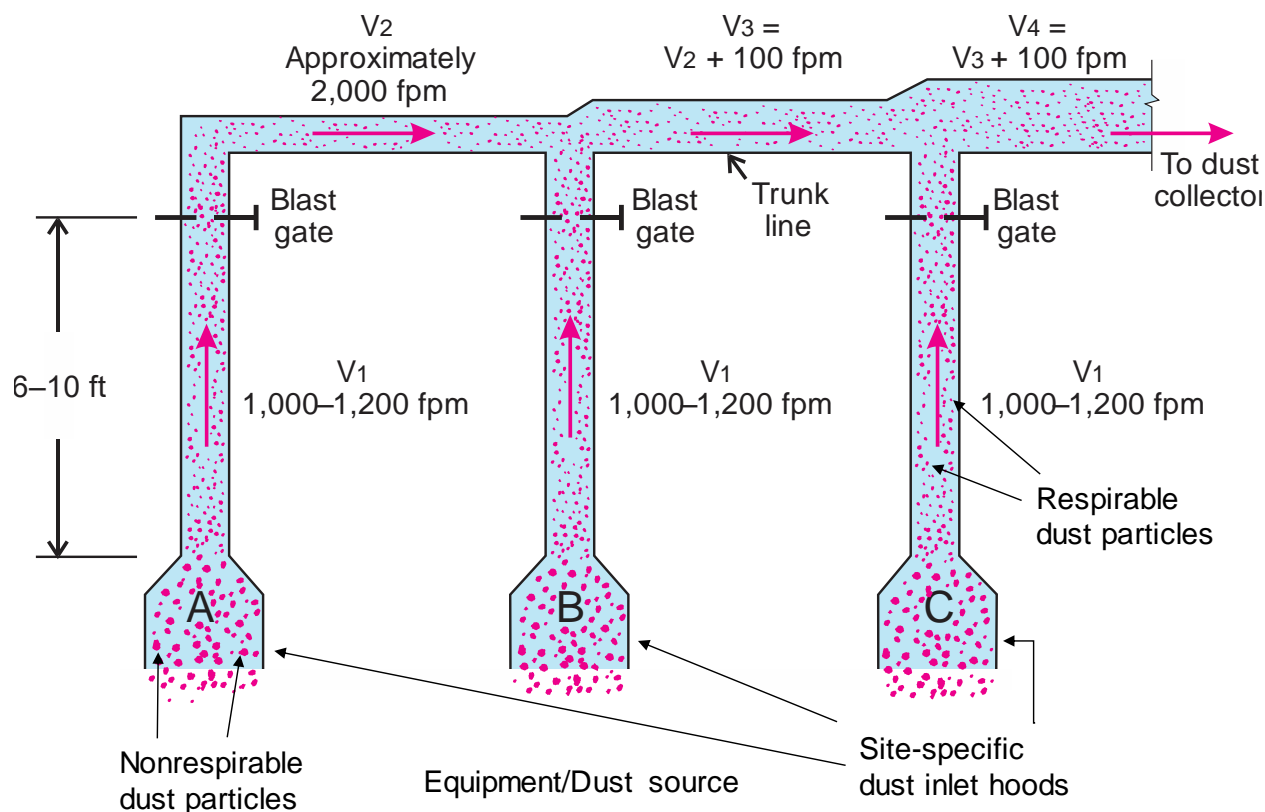
Figure 2.14. Illustration of the horizontal ( V_{2,3,4} ) and vertical ( V_1 ) velocity relationship in a modified low-velocity system. Nonrespirable (larger) dust particles fall back into the process, while respirable (smaller) particles are transported through the ductwork to the dust collector.
