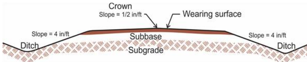
Figure 11.3. Illustration showing a cross section of a haul road. 30
