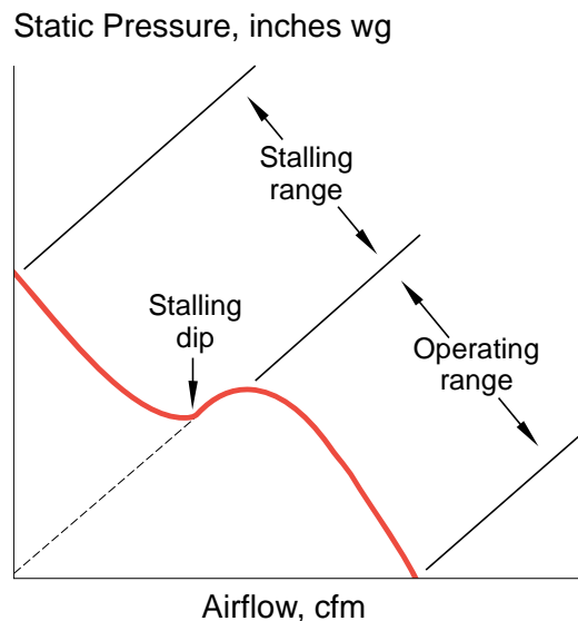
Figure 2.28. Graph of a fan performance curve showing stalling and operating ranges.
