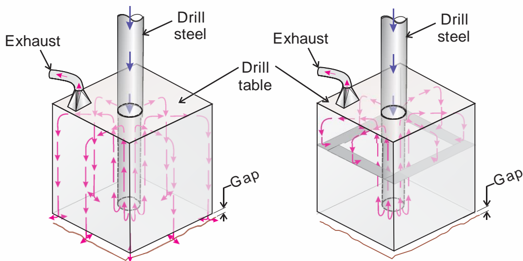
Figure 4.9. Qualitative models of airflow patterns underneath the shroud. The left illustration shows the airflow pattern without the air-blocking shelf. The right illustration shows the airflow pattern with the air-blocking shelf.
