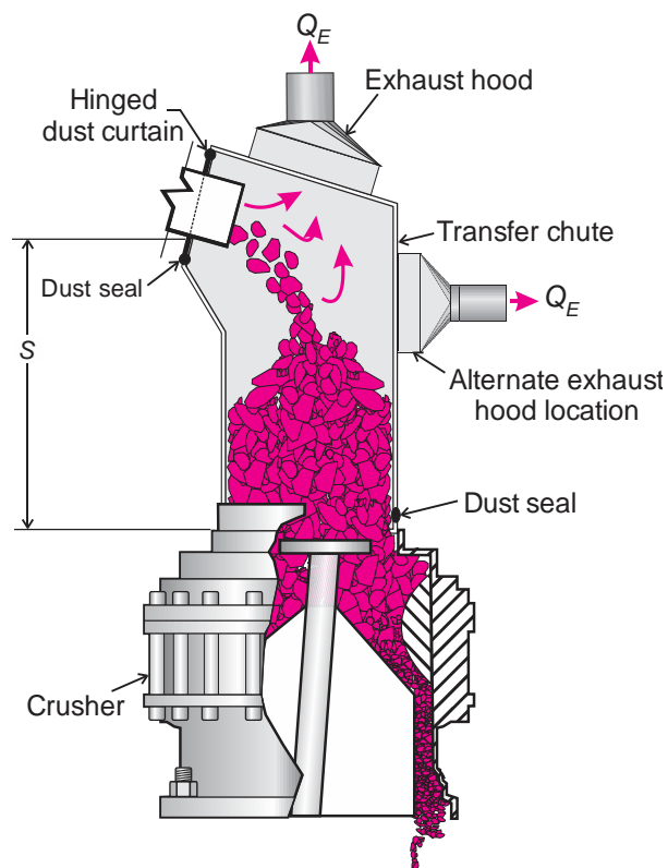
Figure 5.7. Illustration of a dry (exhaust) dust control system on a feed chute into a transfer chute feeding a crusher.
