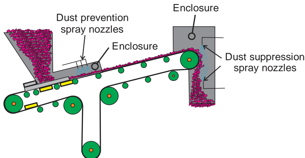
Figure 3.17. Illustration of a typical conveyor dust control application [adapted from Swinderman et al. 2009].
