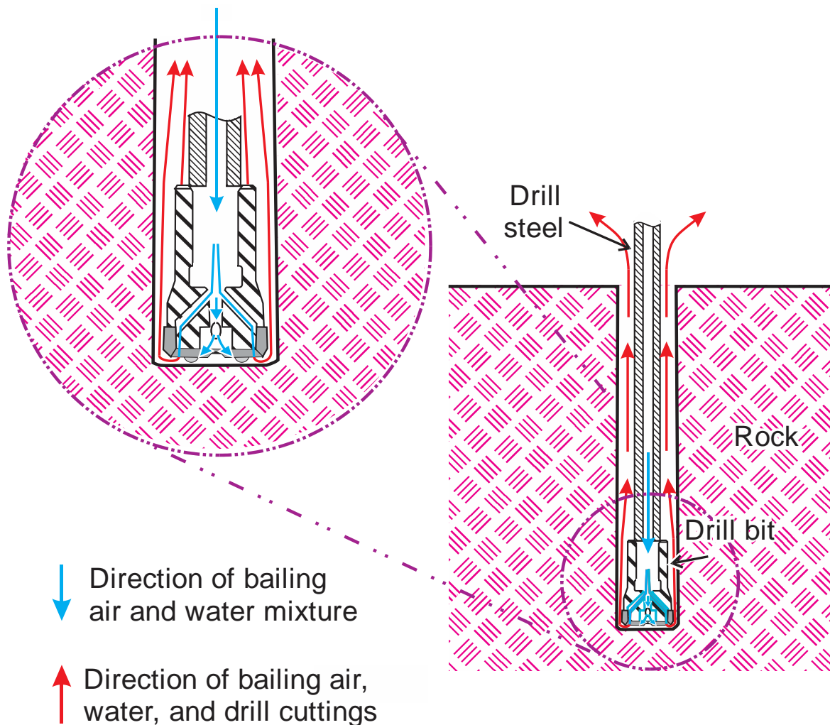
Figure 4.2. Illustration of air and water flow during drilling to demonstrate water flushing of the drill cuttings. The water flows through the center of the drill steel and out the end of the drill bit to remove the cuttings from the drill hole.
