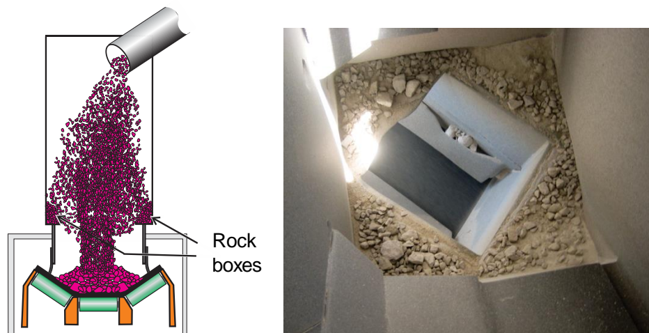
Figure 6.9. Rock boxes used to soften the drop of and redirect the flow of falling material. The left illustration depicts two rock boxes creating a location for ore to accumulate, and the piled ore redirects flow to the center of the belt below. The right photo is an overhead view looking down into the chute, with rock boxes encircling the chute to redirect the ore onto the center of the belt below.
