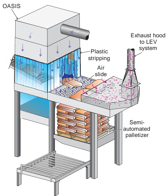
Figure 7.18. Illustration and photo of a semi-automated bag palletizing system. As shown in the left illustration, in this system, a worker removes bags from a conveyor and lifts and positions each layer on an air slide before automated loading onto the pallet. The right photo shows a worker using a semi-automated bag palletizing system, but without plastic stripping. Both an OASIS and an exhaust ventilation system are used to lower the worker's dust exposure during this bag palletizing process.
