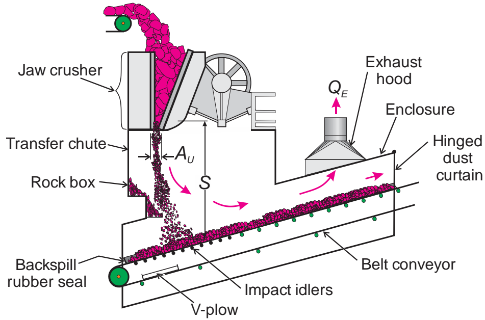
Figure 5.8. Illustration of a dry (exhaust) dust control system at the discharge of a jaw crusher onto a belt conveyor.
