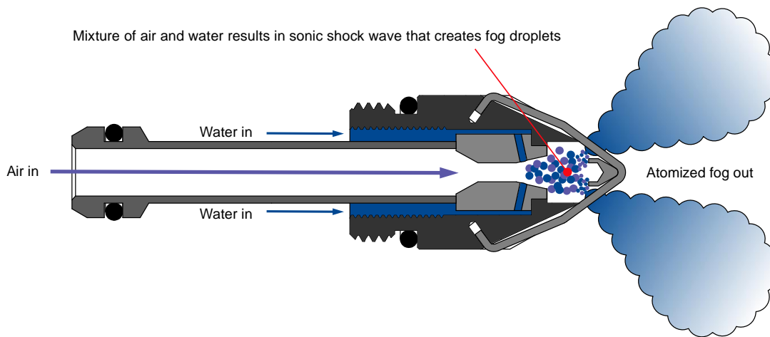
Figure 3.13. Illustration of an ultrasonic dry fog nozzle principle of operation [adapted from Dust Solutions 2018].
