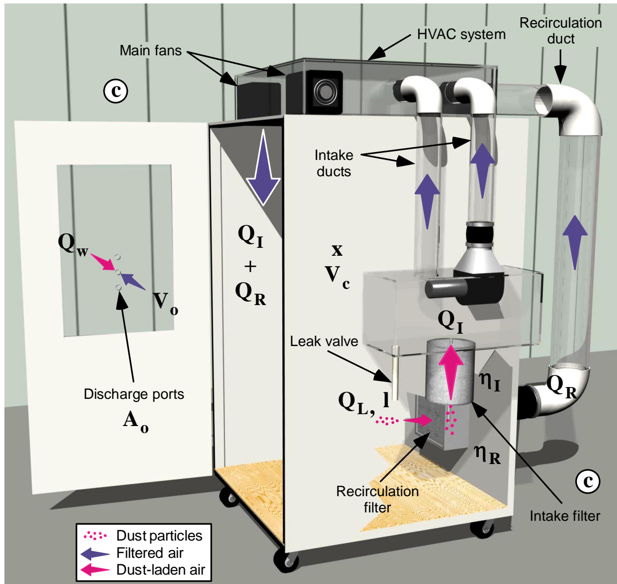
Figure 10.1. Illustration of a simulated enclosed cab tested in the laboratory showing the various test components and parameters for a filtration and pressurization system.
