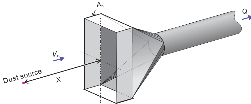
Figure 2.7. Illustration demonstrating the use of a hood entry loss calculation to determine the exhaust volume needed for a basic freestanding hood arrangement [adapted from ACGIH 2010].
