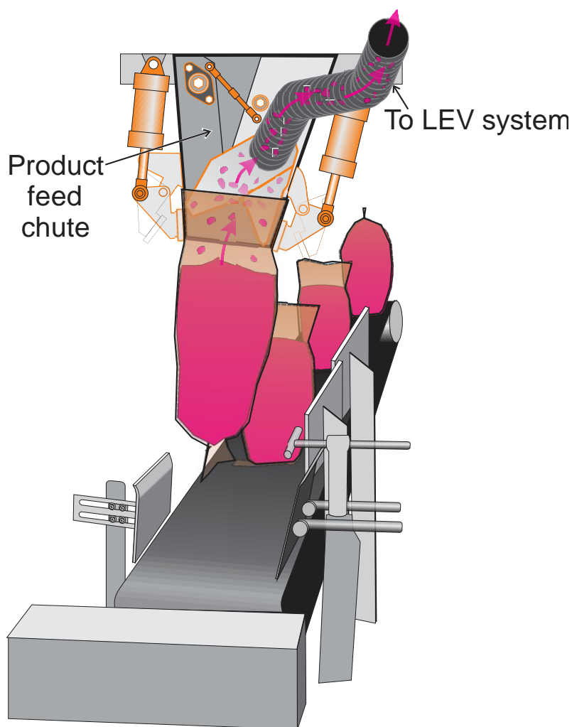
Figure 7.5. Illustration showing an open-top bag being loaded with product. The product is normally whole grain material, which is less dusty.
