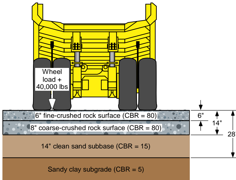
Figure 11.5. Composition and thickness of haul road layers using the California Bearing Ratio [adapted from USBM 1977].
