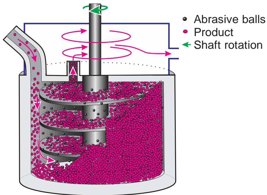
Figure 5.13. Cutaway illustration of a stirring mill.
