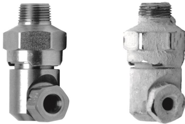
Figure 3.25. Nozzle caking—new versus used [adapted from SSCO 2013].
