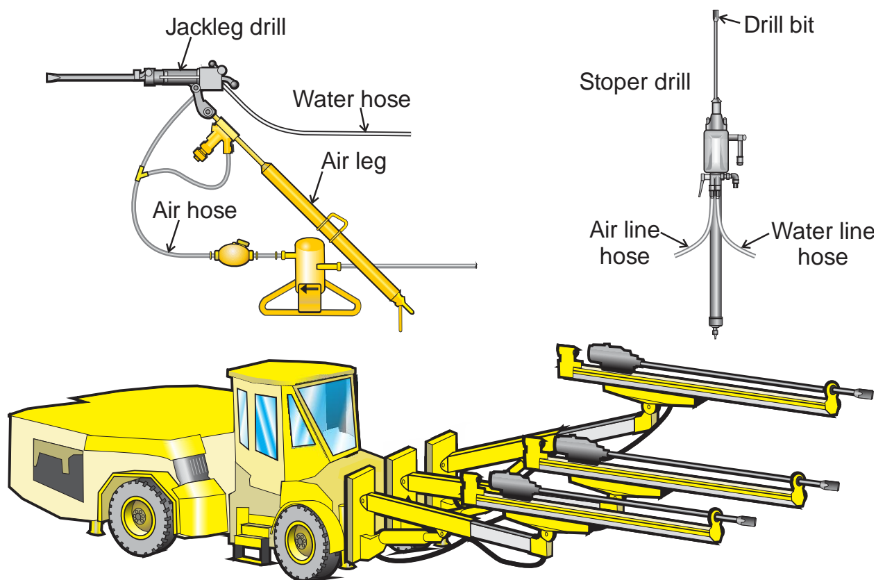
Figure 4.19. Illustrations of three types of drilling equipment. A typical jackleg drill is shown on the top left, a stoper drill on the top right, and a three-boom jumbo on the bottom.
