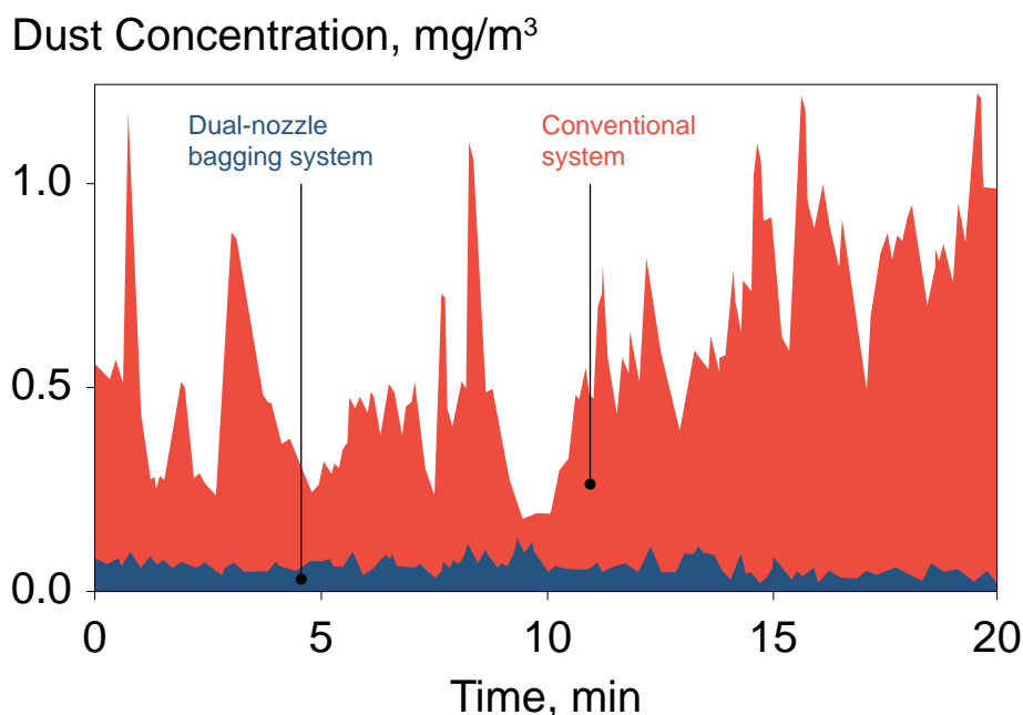
Figure 7.11. Graph showing a bag operator's dust exposure with a conventional (single-nozzle) and dual-nozzle bagging system for a 325 mesh product.
