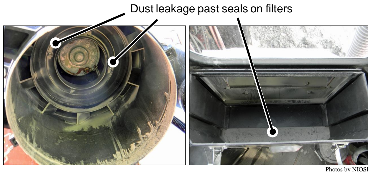
Figure 10.10. Dust leakage path past seals on a canister filter (left) and a panel filter (right).
