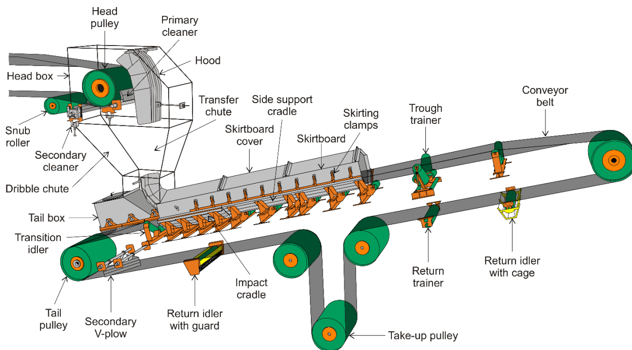
Figure 6.1. Illustration of the basic components of a conveyor belt.
