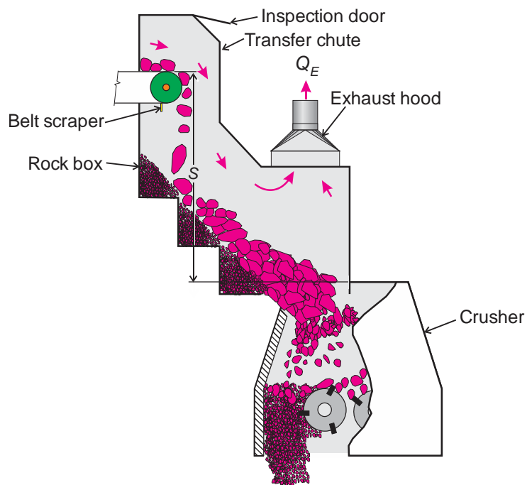
Figure 5.6. Illustration of a dry (exhaust) dust control system at the transfer point of a conveyor discharge to a crusher feed hopper.
