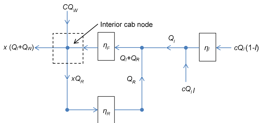
Figure 10.4. Three-filter cab system with the final filter downstream of the intake and recirculation filters. Q's denote air quantities, x's & c's denote contaminant concentrations, and \eta 's denote filter efficiencies.
