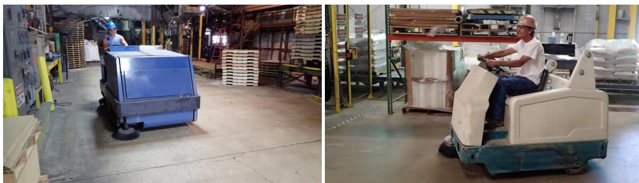
Figure 9.17. Photos of two types of riding floor sweeping units used to clean dust-laden floors. The left photo shows a larger unit with an employee operating from behind. The right photo shows a more compact unit designed for the employee to ride. The size of the unit chosen is based upon plant layout.
