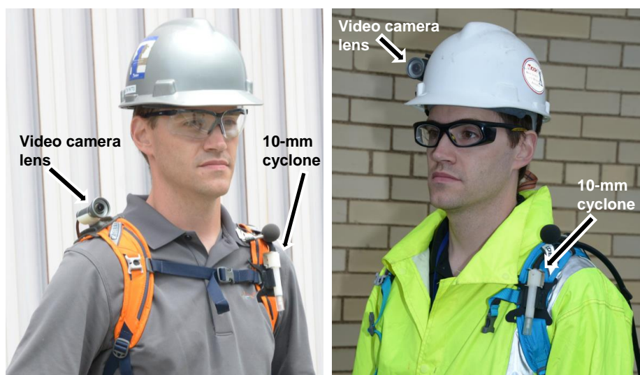
Figure 1.4. Video exposure monitoring options. The left photo shows a video camera lens attached to the worker's backpack shoulder harness and a 10-mm cyclone attached to the shoulder harness. The right photo shows a video camera lens attached to the worker's hardhat and a 10-mm cyclone attached to the shoulder harness.
