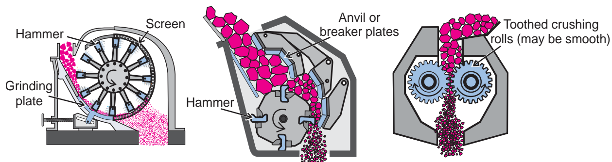
Figure 5.3. Illustrations of three examples of impactive crushers. The left illustration shows a hammermill crusher with material being crushed between the rotating hammers and a fixed grinding plate. The center illustration shows material being crushed between rotating hammers and fixed anvil plates in an impact breaker. The right illustration demonstrates the size-reduction action of a toothed roll crusher.
