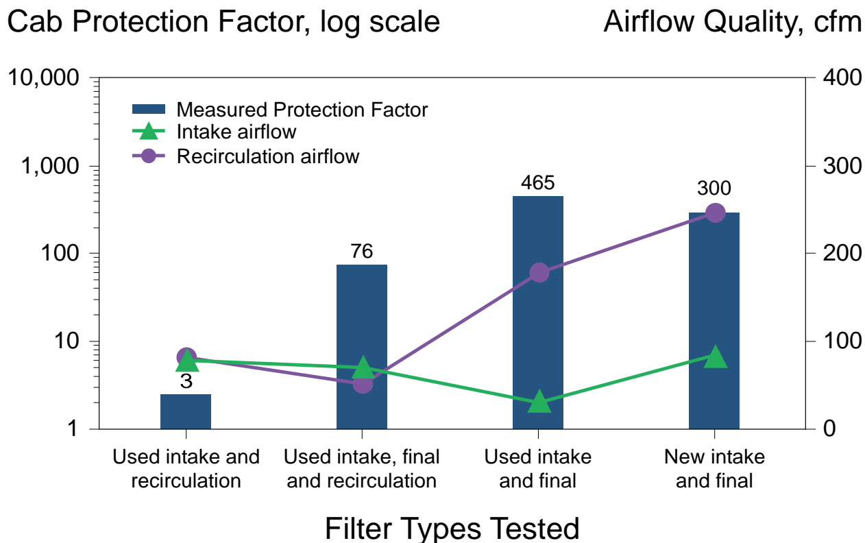
Figure 10.5. Bar chart comparison of cab performance variations with respect to different filters used in a filtration and pressurization system in a field study.
