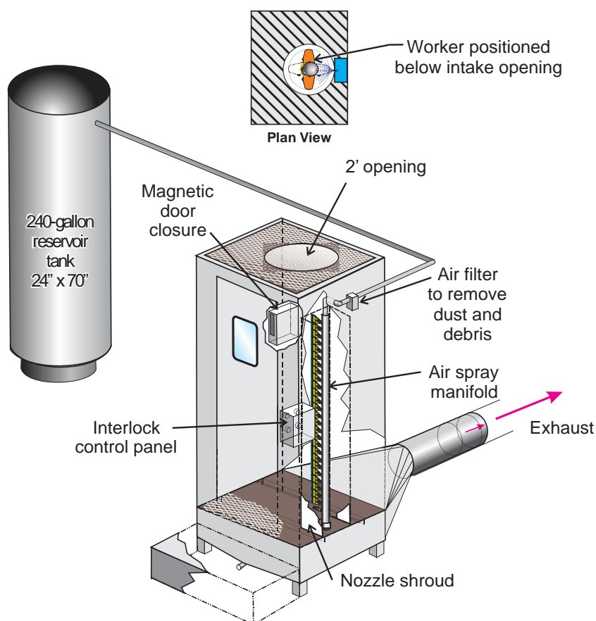
Figure 9.2. Illustration of the overall design of a clothes cleaning system.
