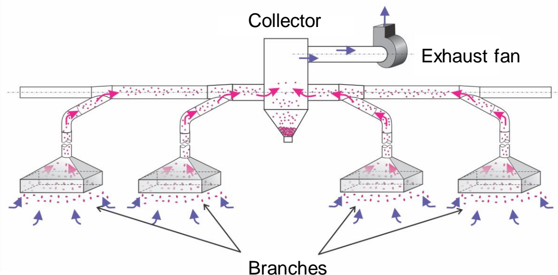
Figure 2.26. Illustration of how a complex exhaust system is a combination of branches linking simple exhaust systems [adapted from ACGIH 2010].
