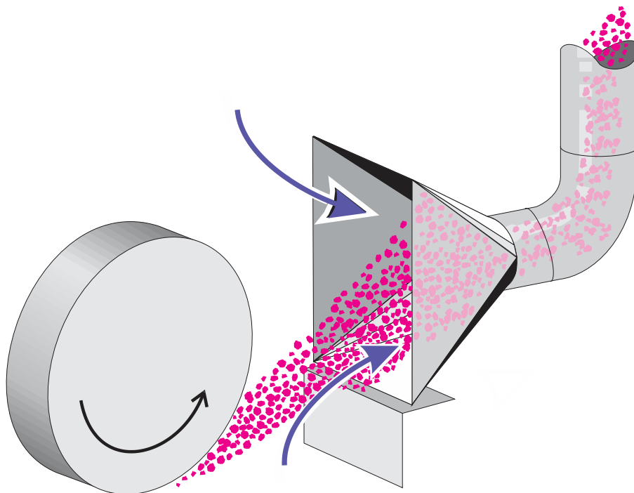
Figure 2.5. Illustration demonstrating a basic setup for a type of receiving hood.
