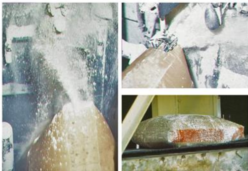
Figure 7.1. Dust sources during bagging. The left photo shows product “rooster tail.” The top right photo shows product blowback. The bottom right photo shows dust-soiled bag.
