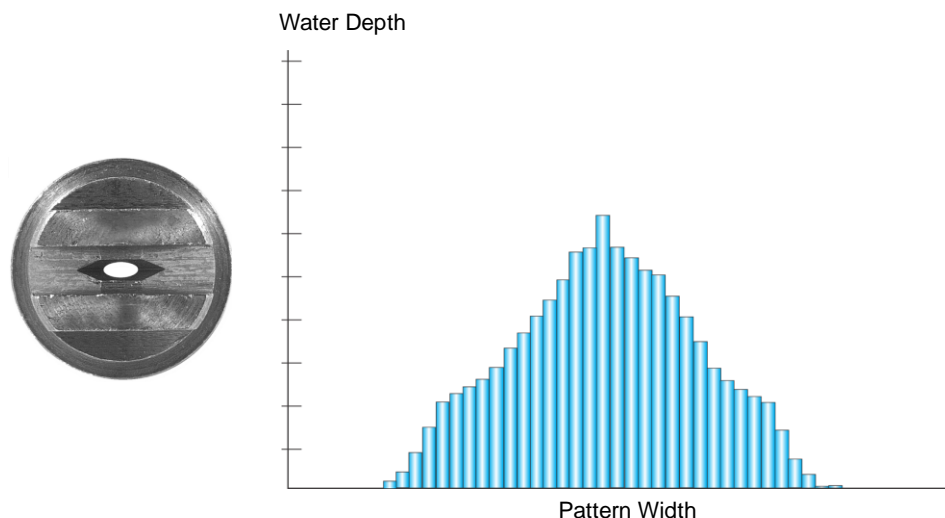
Figure 3.29. Worn spray tip showing pattern and distribution graph. Bar height indicates distribution of water over pattern width and shows an increase of and excessive flow in the center of the pattern due to orifice wear [adapted from SSCO 2013].
