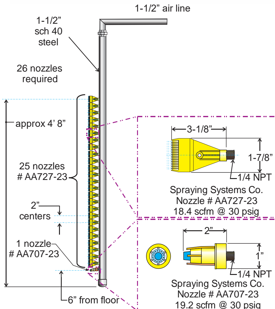
Figure 9.3. Air spray manifold design with 26 nozzles spaced two inches apart.
