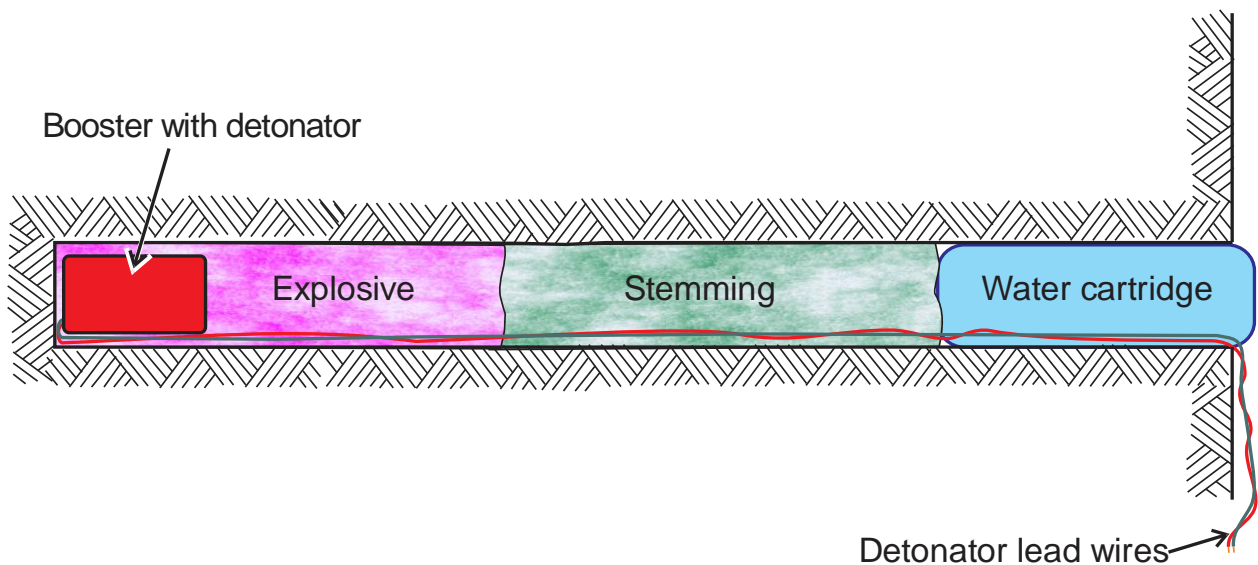
Figure 4.22. Illustration of a typical blasthole containing an explosive charge with stemming and using a water cartridge to suppress dust.
