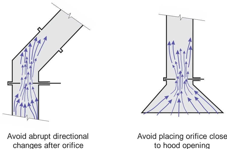
Figure 2.13. Illustration demonstrating poor orifice plate placement.
