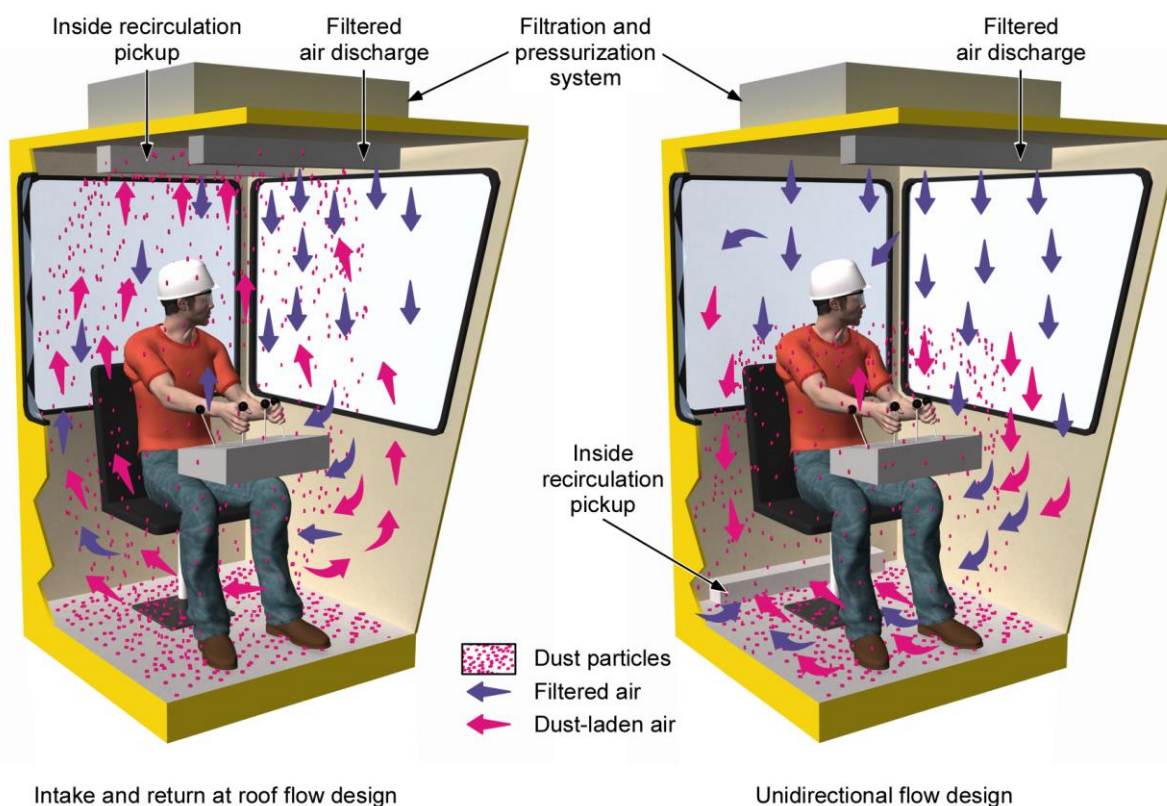
Figure 10.18. Illustration of the airflow pattern for intake and return at the roof of a cab and a unidirectional airflow design.
