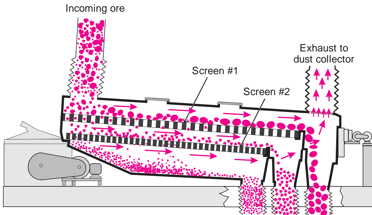
Figure 5.16. Illustration of a dry (exhaust) dust control system on a vibrating screen.
