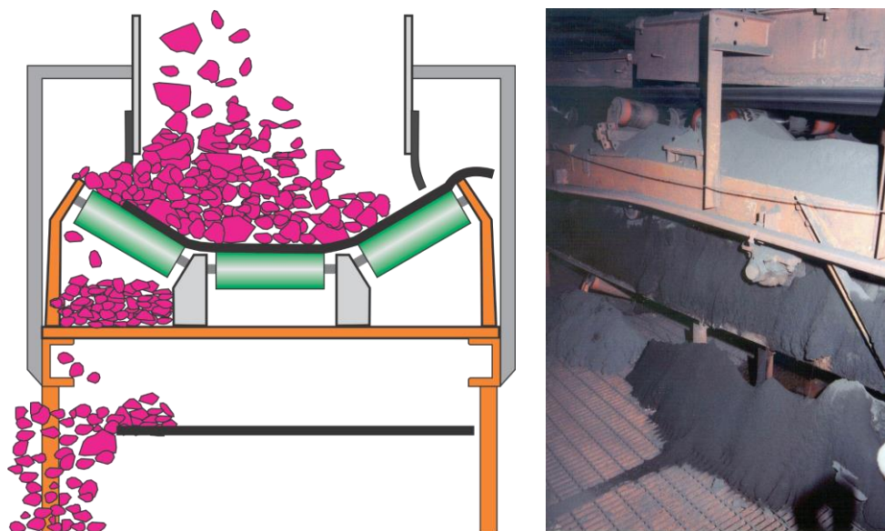
Figure 6.3. Example of material spillage from a conveyor belt, which is a safety hazard and a source of dust, and which causes premature equipment wear. The left illustration shows material spillage below the belt, causing equipment wear. The right photo shows major ore spillage from a belt, which will result in premature wear and more frequent repair. This spillage is also a constant source of respirable dust exposure to workers in the vicinity of the belt.
