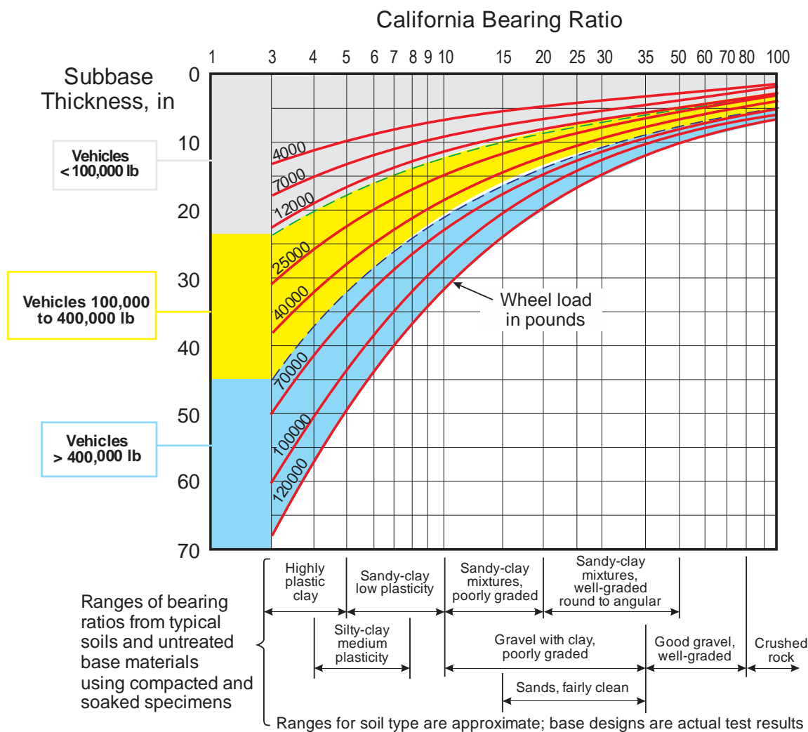
Figure 11.4. Subbase thickness from California Bearing Ratio tests on road material [from USBM 1977].
