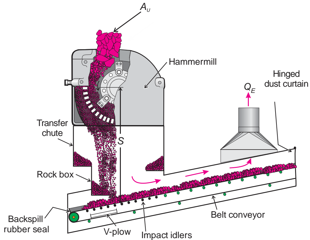
Figure 5.9. Illustration of a dry (exhaust) dust control system at the discharge of a hammermill crusher onto a belt conveyor.
