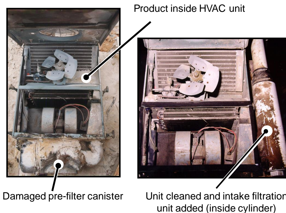
Figure 10.13. Damaged filtration units, representing poor housekeeping. The left photo shows a filtration unit with an obvious lack of maintenance and care, and the right photo shows the unit after cleaning and with the addition of a new intake air filtration unit.
