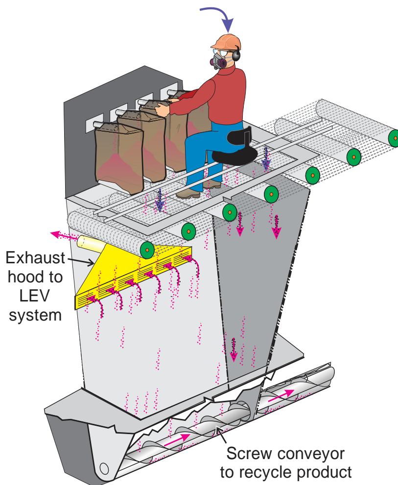
Figure 7.9. Illustration of an exhaust hopper below a bag loading station with an integrated LEV system to capture dust generated during the bag loading process.
