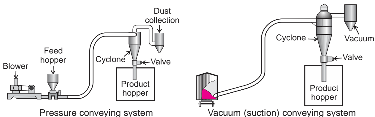
Figure 6.25. Illustration of two types of pneumatic conveying systems.
