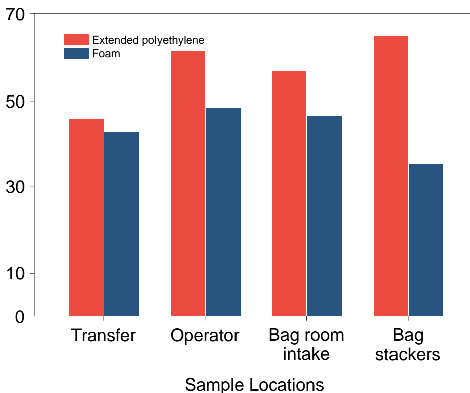
Figure 7.7. Bar chart showing dust reductions with extended polyethylene and foam valves as compared with the use of the standard paper valve.
