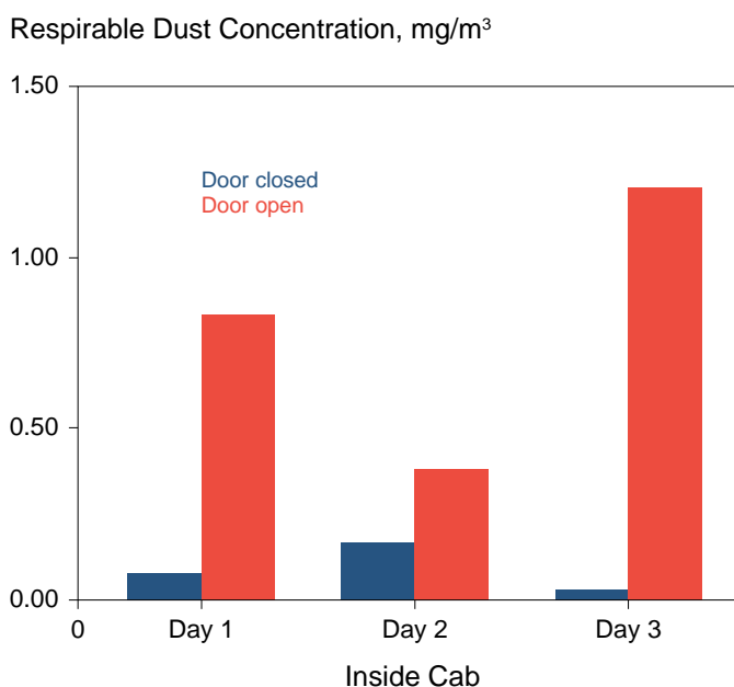
Figure 10.11. Bar chart showing respirable dust concentrations inside an enclosed cab for three days of testing with the cab door closed and open. The photo shows the operator opening the cab door and significantly increasing his exposure, even though drilling had ceased two minutes earlier.
