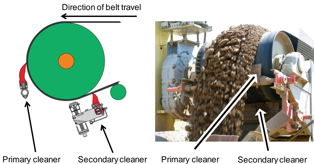
Figure 6.18. Primary and secondary cleaners used to scrape material from a belt. The left illustration shows the location of the primary and secondary cleaners in relation to the head pulley and belt. The right photo shows ore being discharged from the belt with the primary and secondary cleaners in action.
