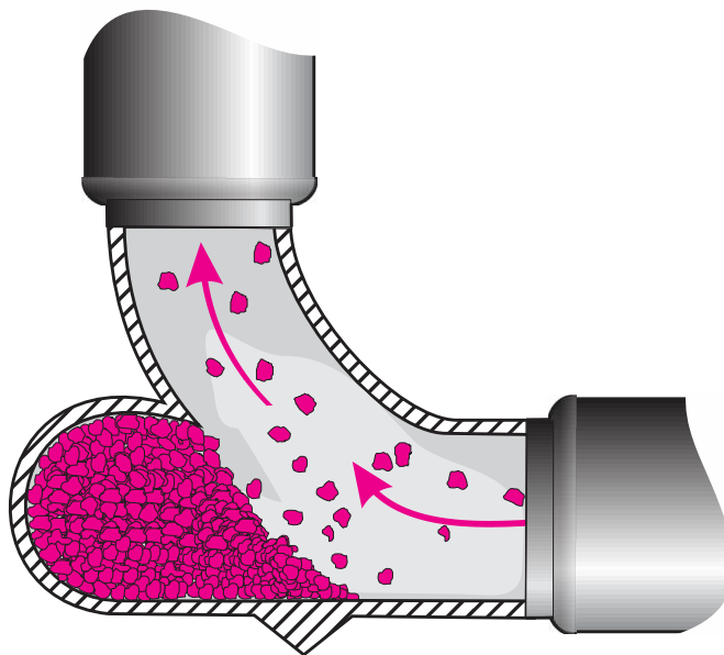
Figure 6.26. Illustration of a wear-resistant elbow installed in conveying ductwork.
