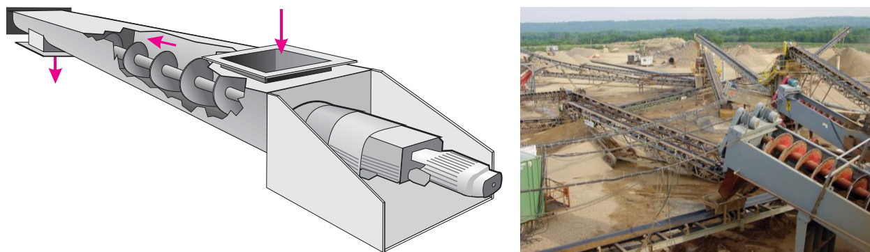
Figure 6.22. Screw conveyors designed to move material through a stationary trough. The left illustration shows a typical screw conveyor, with arrows representing the direction of material flow. The right photo depicts two screw conveyors installed at a mining operation.
