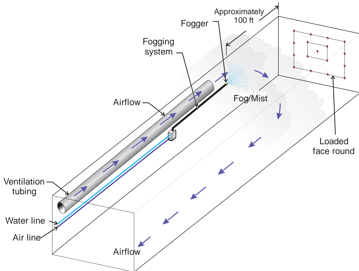
Figure 4.23. Illustration of a fogger spray used to create a mist for dust suppression in the heading where blasting will occur.
