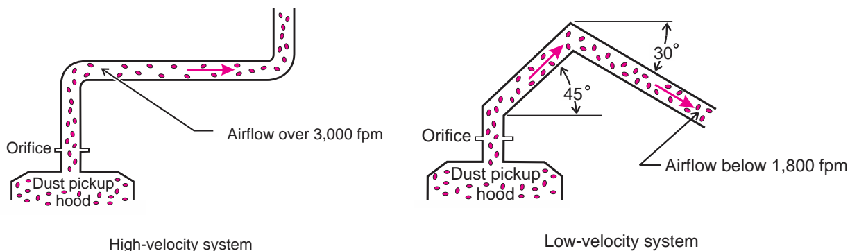
Figure 2.9. Illustration depicting the basic differences between high- and low-velocity systems.
