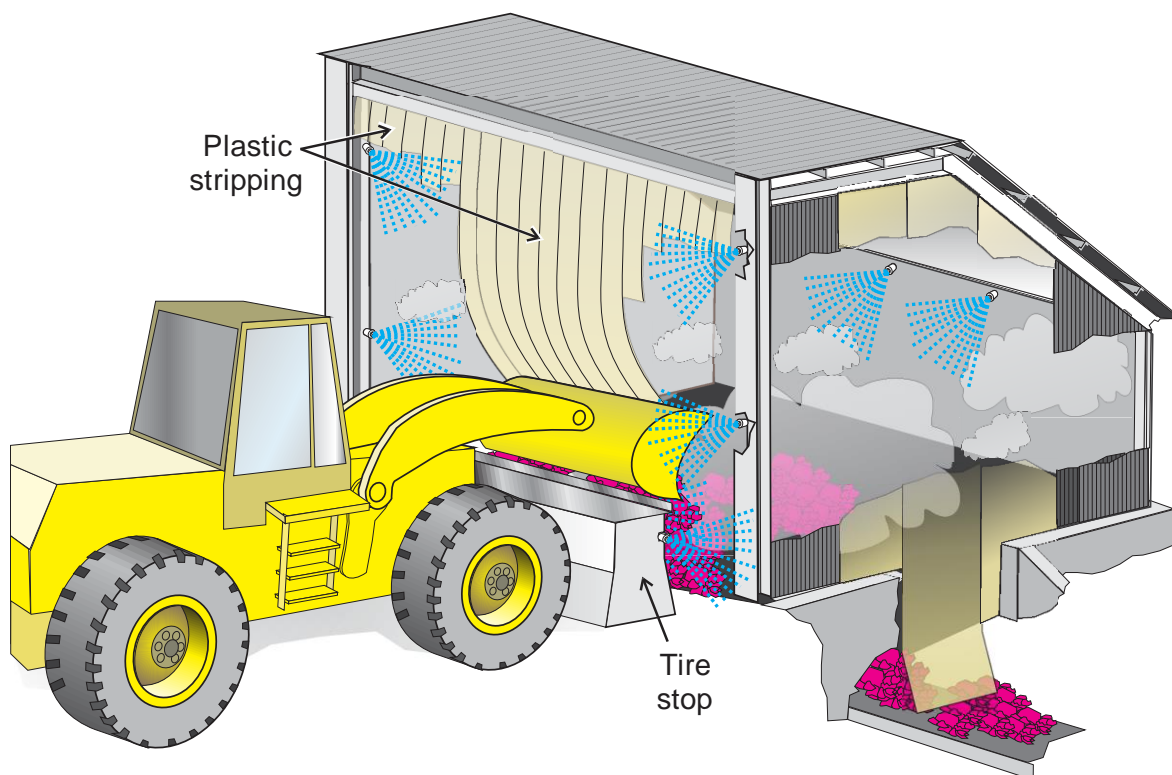
Figure 5.4. Illustration of a wet dust control approach with a partial enclosure at a crusher dump loading operation. Note the blue “fan patterns” signifying water sprays.
