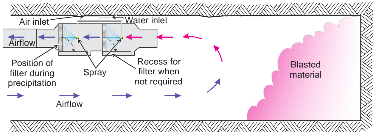
Figure 4.25. Illustration of a filtration unit, located in the blast heading, used for filtering contaminated ventilation air from the blast heading after blasting occurs.
