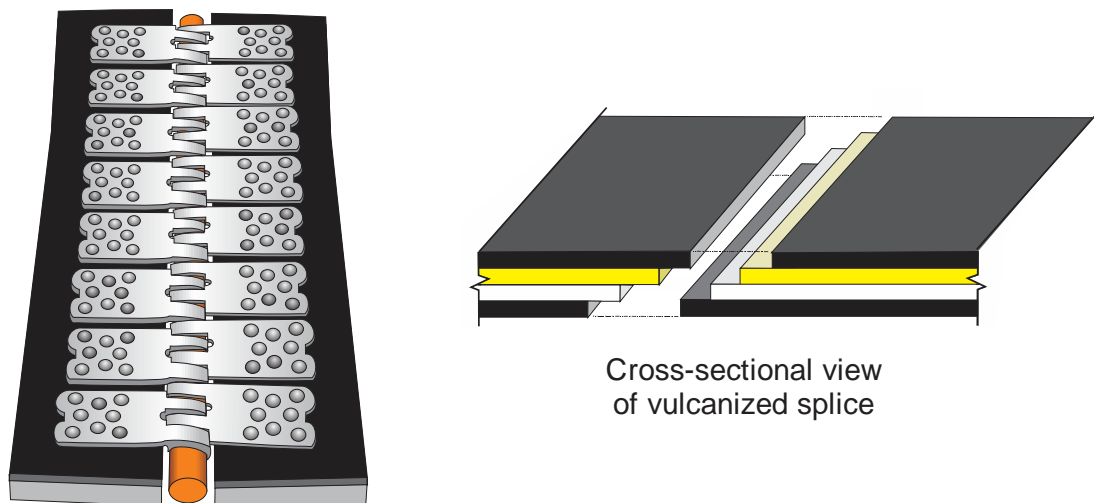
Figure 6.21. Illustration of a mechanical belt splice (left) and a vulcanized belt splice (right).
