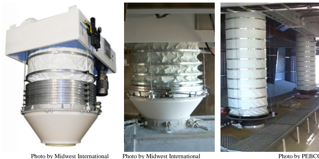
Figure 8.2. Photos of loading spout discharge cones designed to seal against the loading port of closed vehicles to minimize dust liberation.
