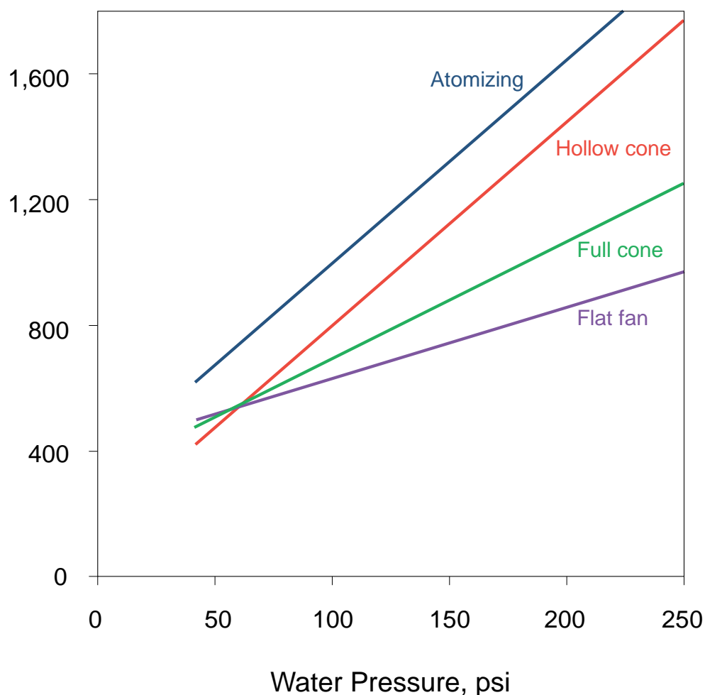
Figure 3.11. Airborne suppression performance of four types of spray nozzles. The atomizing nozzle is air atomizing. The hollow cone, full cone, and flat fan spray nozzles are hydraulically atomizing [adapted from NIOSH 2003].
