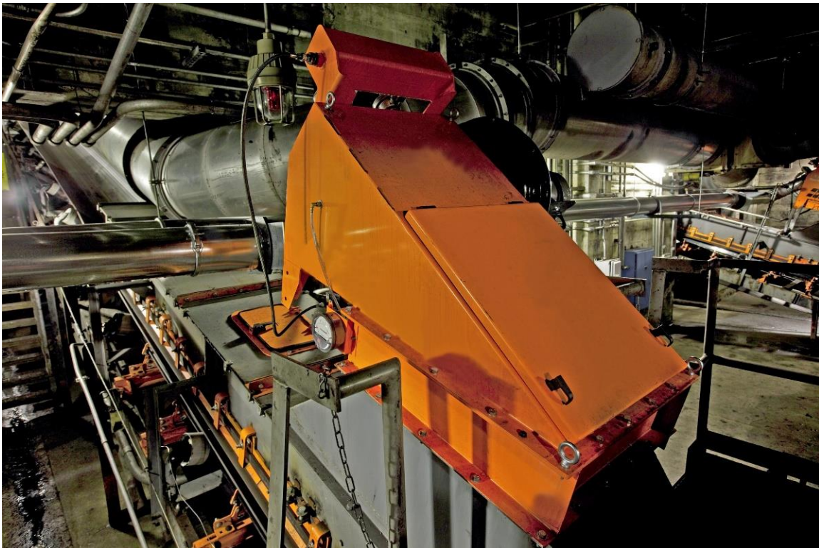
Figure 6.17. A conveyor transfer point enclosure used with an exhaust ventilation system. The top illustration shows some of the key design considerations. The bottom photo shows an exhaust ventilation system (air cleaner) mounted on top of a transfer system.
