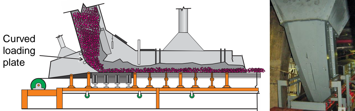
Figure 6.10. A curved loading plate (spoon) to help steer loaded material in a particular direction. The left illustration shows the curved loading plate within a chute. The right photo shows an end view of a curved chute.
