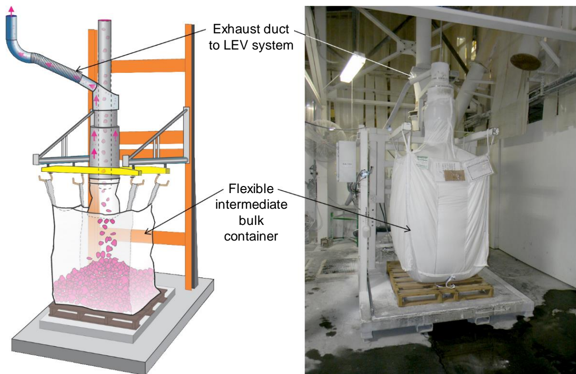
Figure 7.23. Illustration and photo of exhaust ventilation system being used during the loading of flexible intermediate bulk containers.
