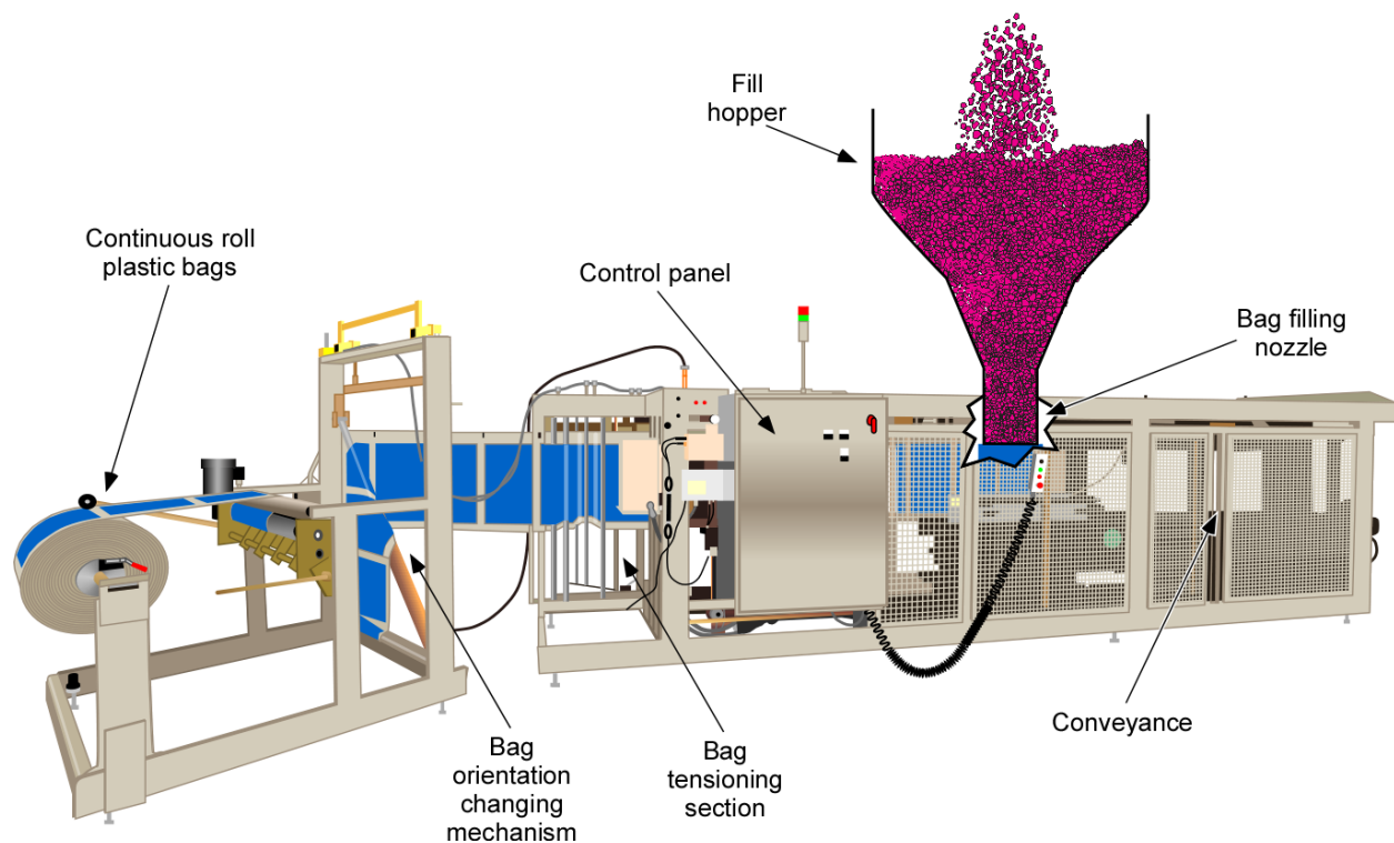
Figure 7.14. Illustration of a form-fill-seal (FFS) machine. The process moves from left to right, starting with the bag supply, re-orientation and tensioning, fill hopper, and belt transfer to the stacking area. (LEV system not shown.)
