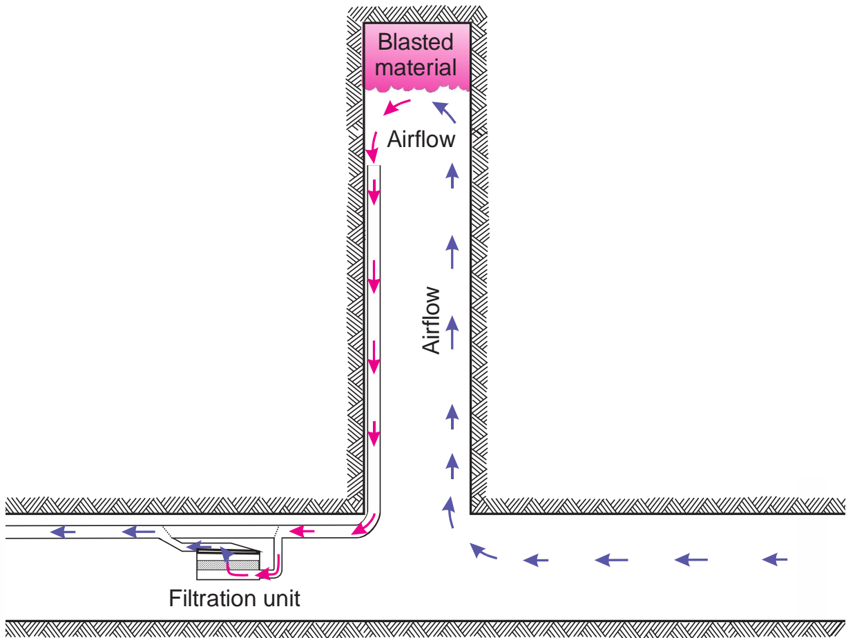
Figure 4.24. Illustration of a filtration unit, located adjacent to the blast heading, used for filtering contaminated ventilation air from the blast heading after blasting occurs.
