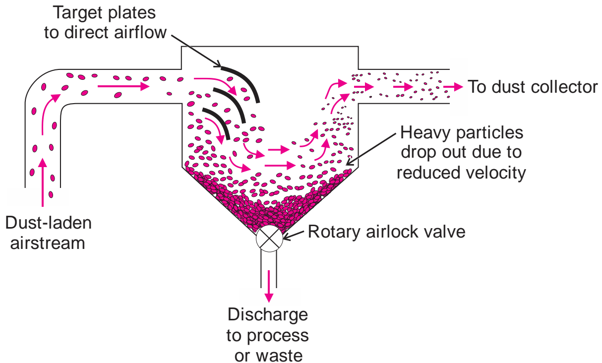
Figure 2.15. Illustration showing a typical design of a gravity separator (drop-out box).
