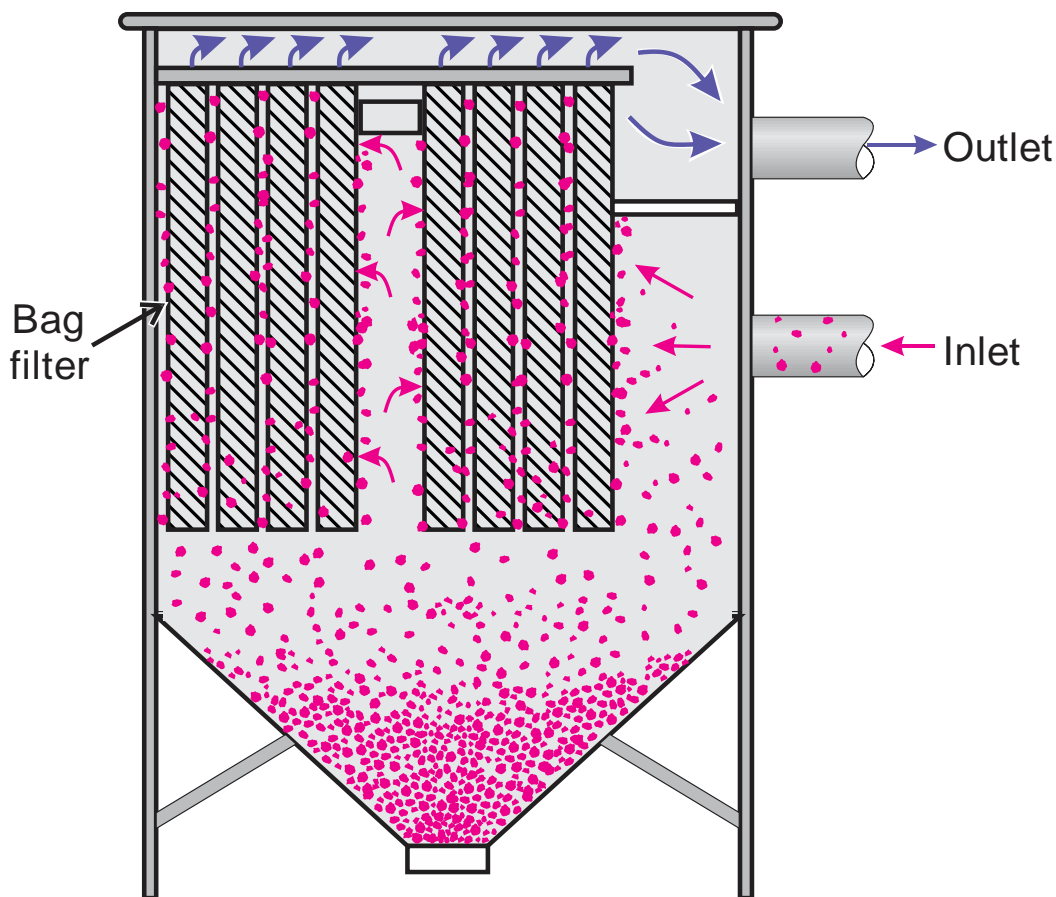
Figure 2.17. Illustration showing a basic design of a baghouse dust collector.
