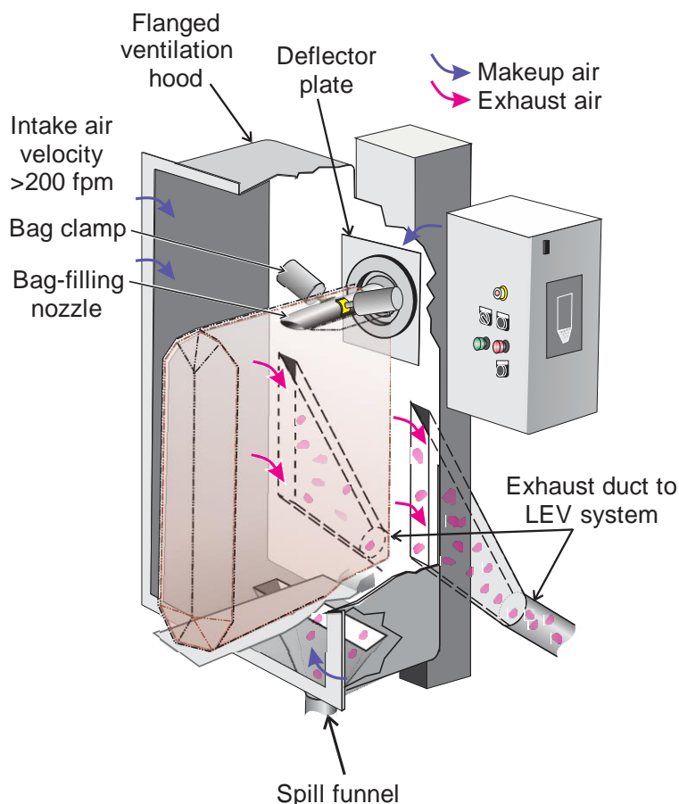
Figure 7.8. Illustration of exhaust shrouding to capture and exhaust respirable dust away from each fill nozzle.
