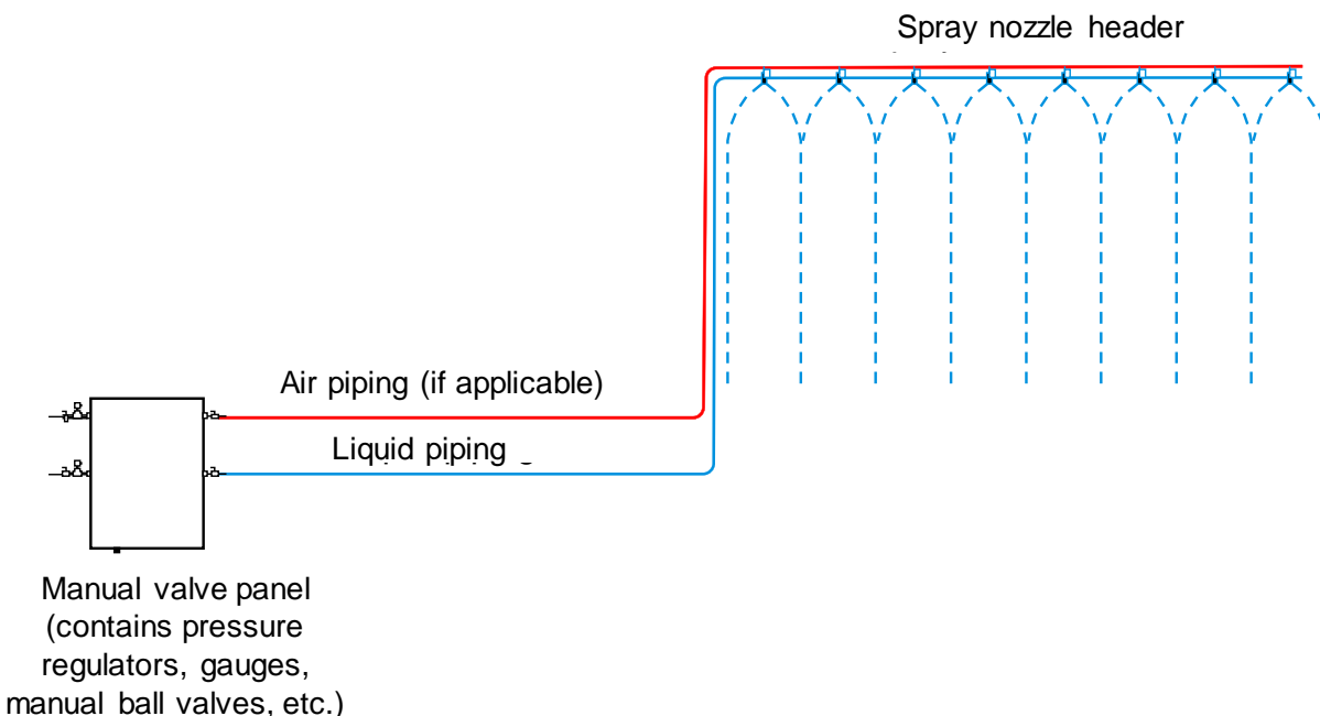
Figure 3.18. Illustration of a typical manual valve control system schematic.
