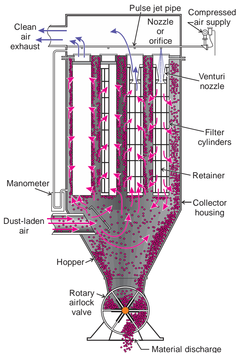
Figure 2.20. Illustration of a typical design of a pulse jet dust collector.
