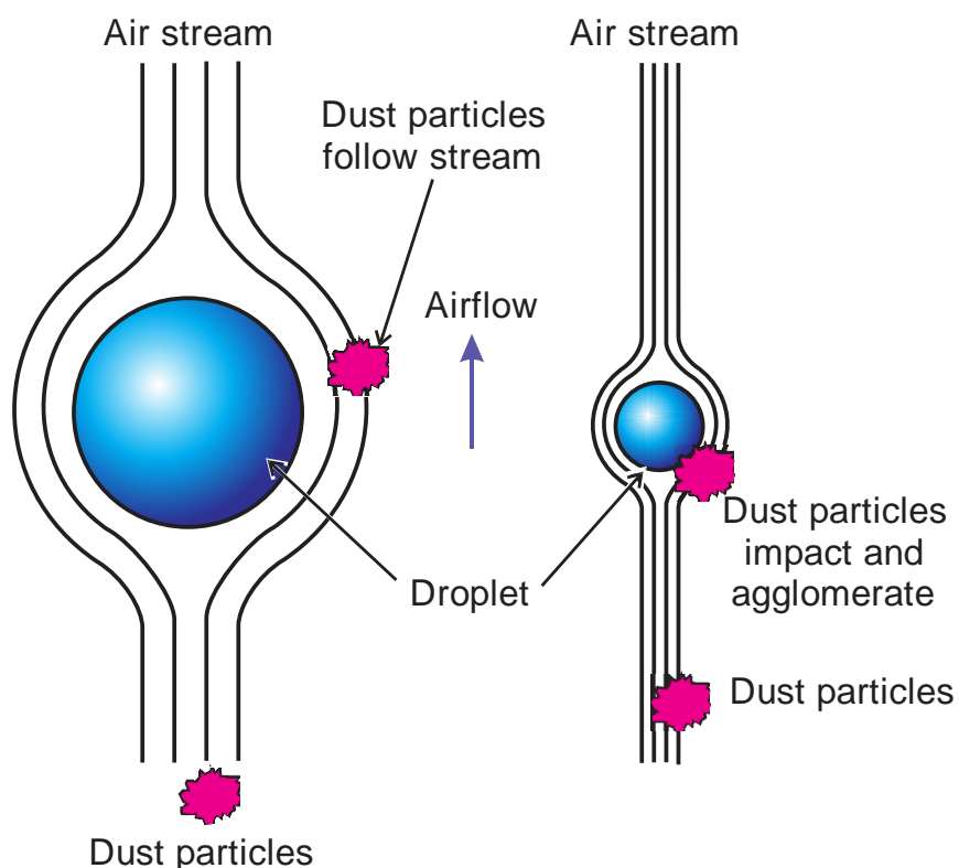
Figure 3.3. Illustration of the effect of droplet size on dust particle impingement.
