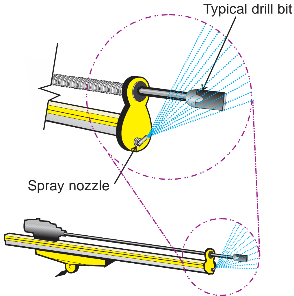
Figure 4.21. Illustration of drill boom showing external water sprays directed onto the drill steel and toward the collar of the hole.
