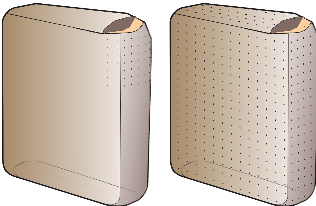
Figure 7.3. Two types of bag perforations. The left illustration shows undervalue perforations. The right illustration shows overall perforations.
