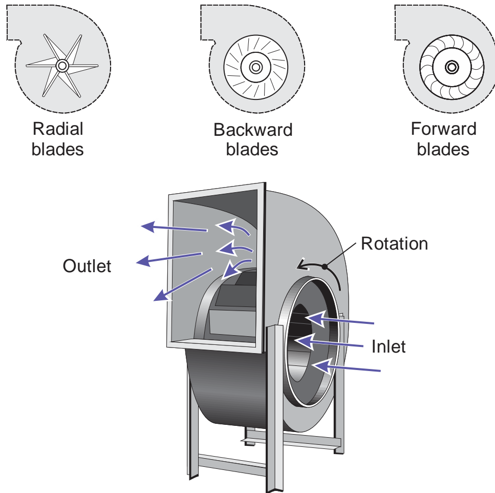
Figure 2.31. Illustration of a typical centrifugal fan.
