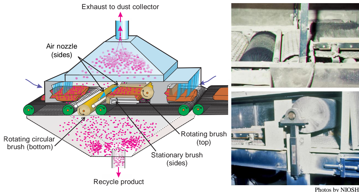
Figure 7.16. Illustration and photo of a bag and belt cleaning device. The left illustration shows the overall device design, with the magenta arrows indicating a closed system under negative pressure. The right photos show stationary (top) and rotating (bottom) brushes in actual service.
