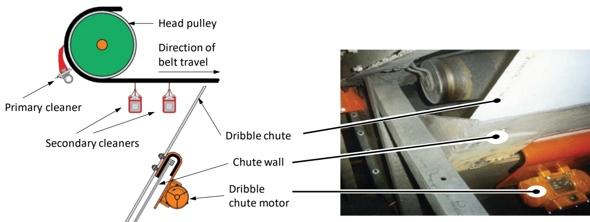
Figure 6.19. Illustration of a dribble chute applied to return material to belt flow.
