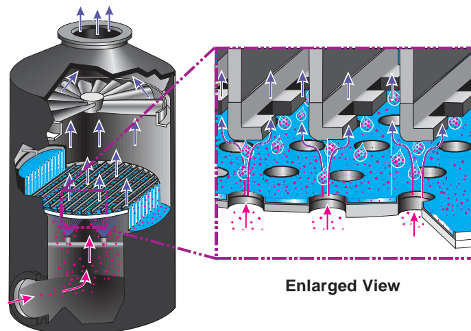
Figure 2.24. Illustration showing a typical design of an impingement plate scrubber.
