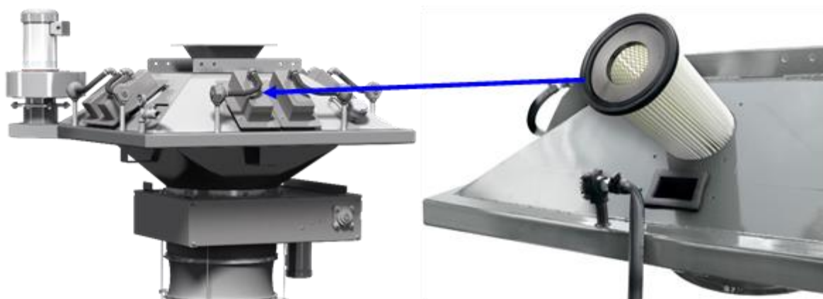
Figure 8.5. Photos of a top-mounted dust collection unit and an expanded view to show filter cartridge access.
