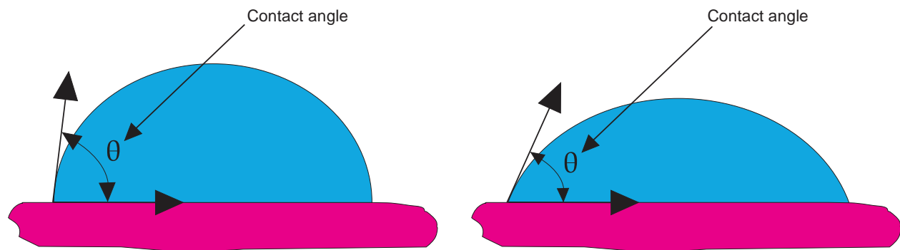
Figure 3.4. Illustration of contact angle resulting from a liquid meeting a solid surface. The left image shows a non-treated water droplet with a greater contact angle. The right image shows a surfactant-treated water droplet with a lesser contact angle [adapted from NDT 2018].
