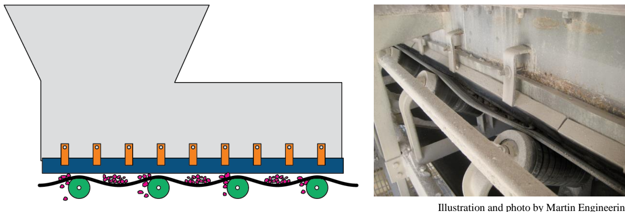
Figure 6.11. Material spillage and entrapped fugitive material resulting from belt sag. Both the left illustration and the right photo show belt sagging between idlers.
