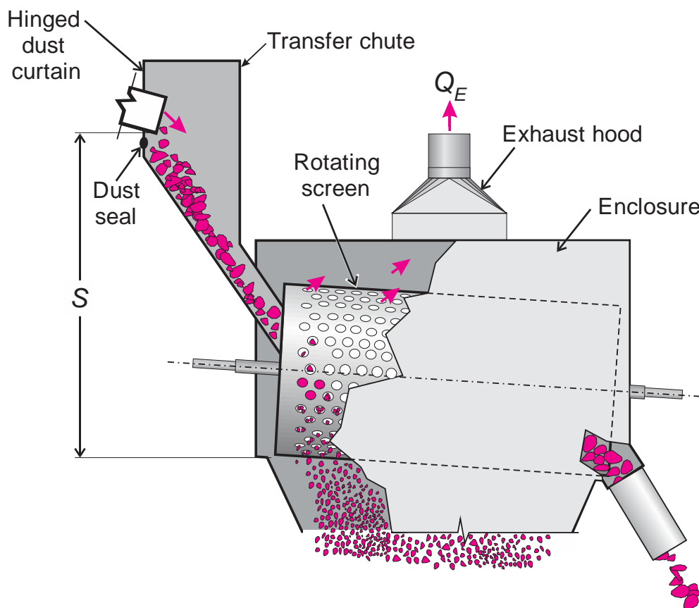
Figure 5.15. Illustration of a dry (exhaust) dust control system on the feed to a rotary screen with an enclosed transfer chute. See Equation 5.2 for a definition of variables.
