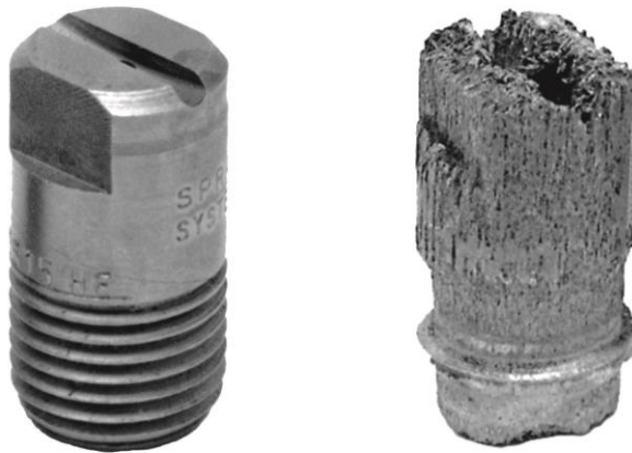
Figure 3.24. Nozzle corrosion—new versus used [adapted from SSCO 2013].
