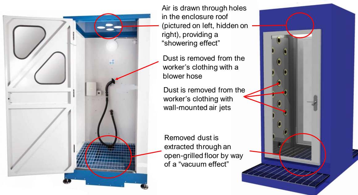
Figure 9.6. Two clothes cleaning systems using high-velocity air through a blower system for removing contaminants from work clothing. Though these systems are made by different manufacturers, they have some common features, as noted in the labels.
