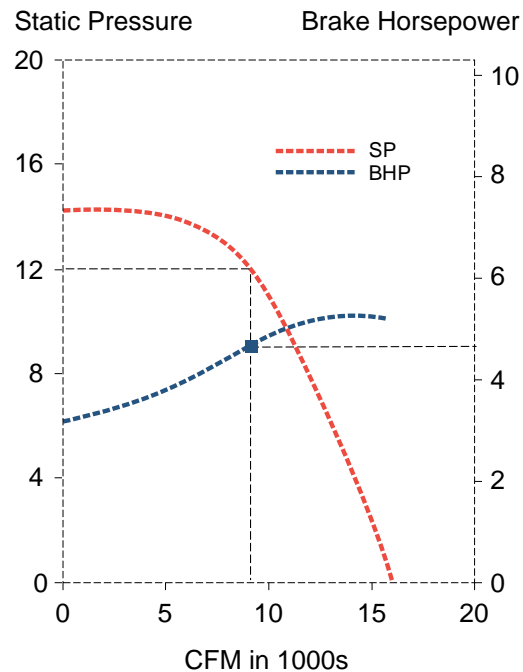
Figure 2.27. Graph of a typical fan performance curve. Each fan curve is associated with a certain fan model at a selected RPM.
