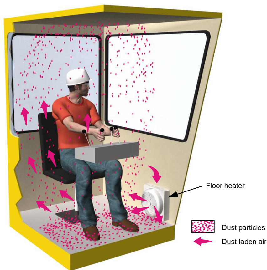
Figure 10.12. Illustration of the problem created by a heater stirring up dust from the floor and blowing dust off of the worker's clothing.
