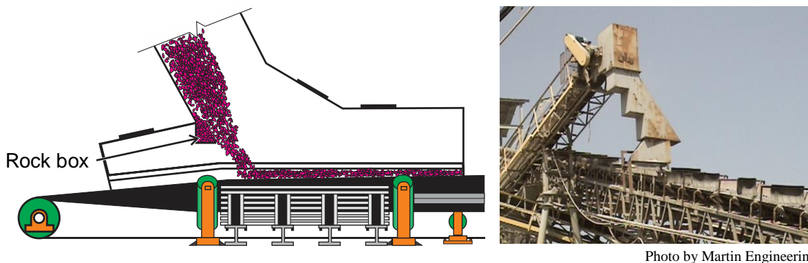
Figure 6.6. Rock boxes used to minimize impact of falling material. The left illustration shows a rock box softening the load by reducing the drop height, with ore used as the deflection mechanism in order to reduce wear on metal parts. The right photo shows a series of rock boxes redirecting the material from one belt onto the next belt.
