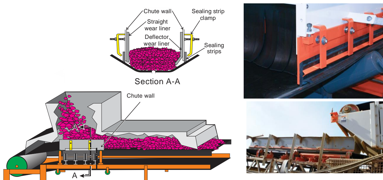
Figure 6.12. Wear liner and chute wall installed near the belt and within a transfer zone to maintain the loaded ore on the belt. The left illustration shows a transfer zone of a belt with a cutaway (Section A-A) view of the chute wall, the wear liner, the sealing system, and the belt. The top right photo shows an actual application of the chute wall, wear liner and sealing system, which includes a sealing strip and clamp system. The bottom right photo shows a transfer zone application in the field.
