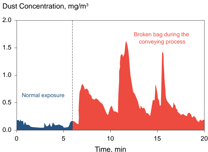
Figure 9.23. Graph showing the increase in a worker's respirable dust exposure from a broken bag during the conveying process.
