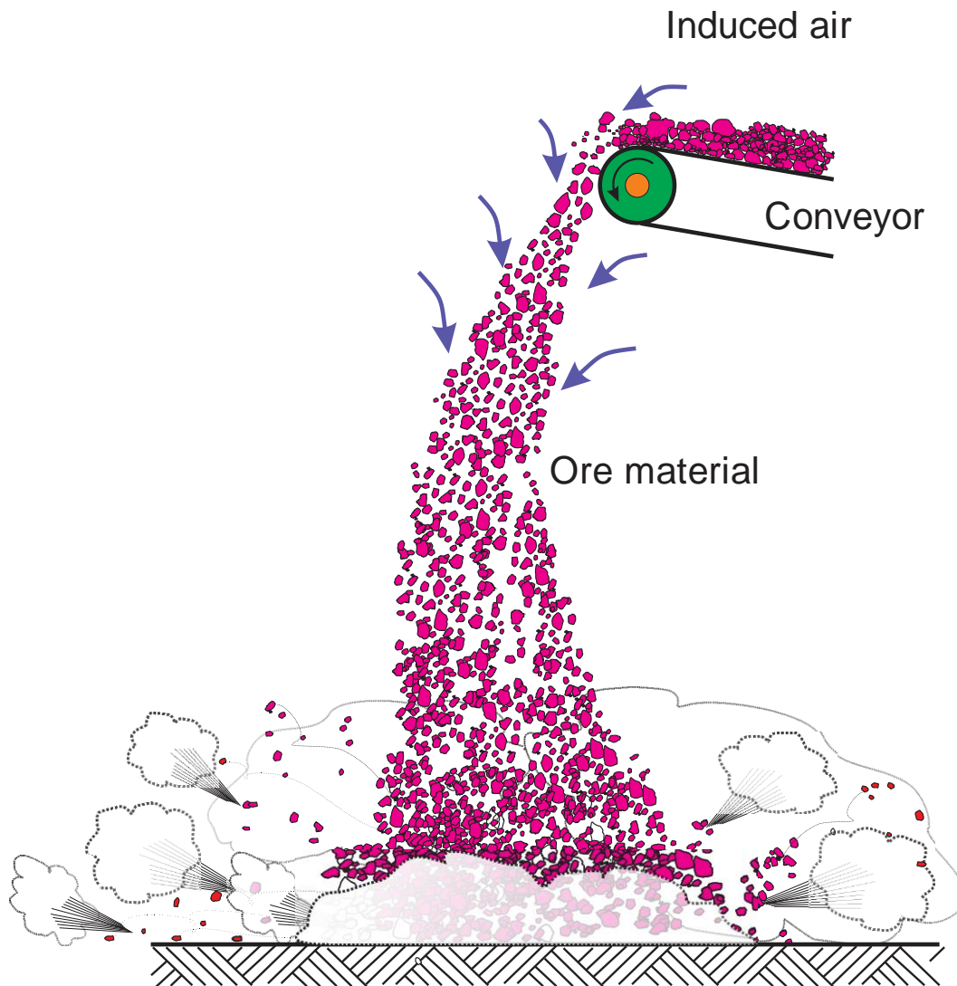
Figure 2.6. Illustration demonstrating air induction as material falls from a conveyor.
