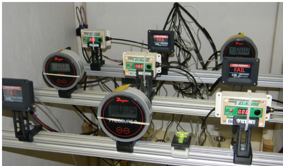
Figure 10.15. Comparison of three different types of pressure gauges in an experimental filtration laboratory test booth.
