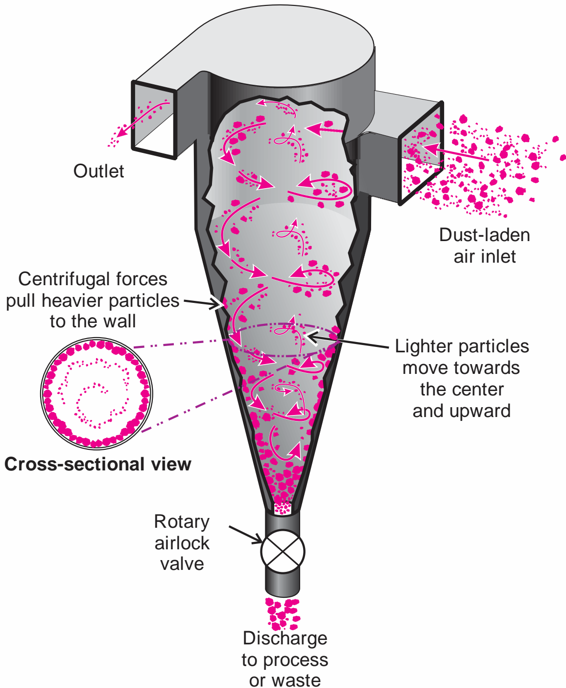
Figure 2.16. Illustration showing a typical design of a cyclone dust collector.
