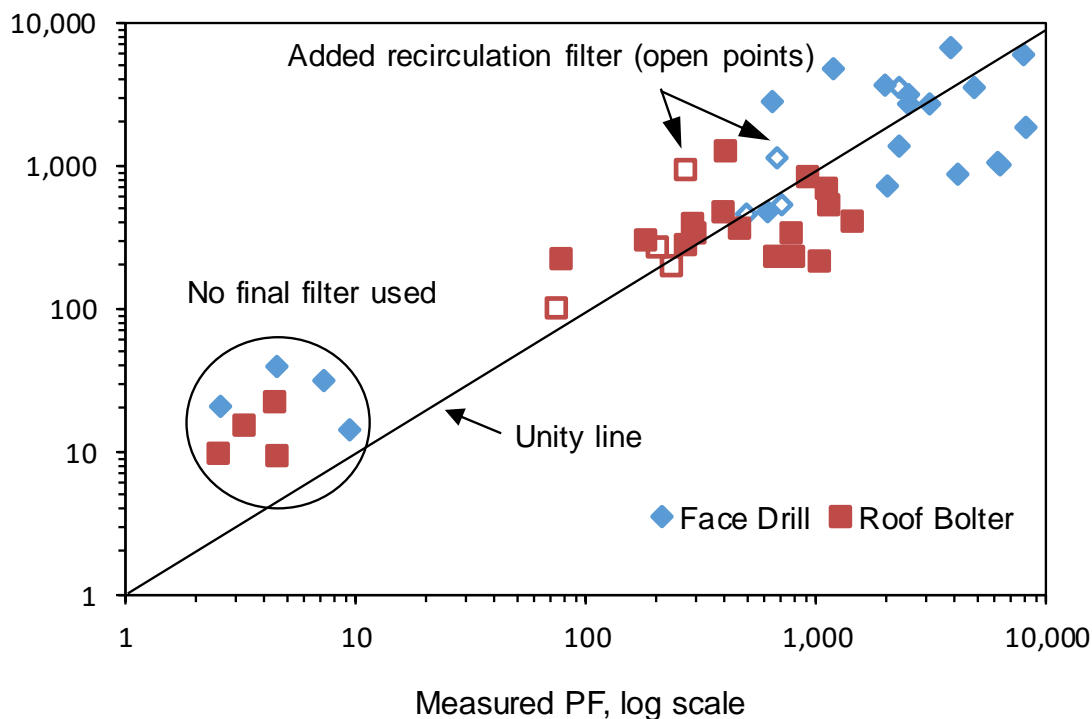
Figure 10.9. Graph showing the measured and modeled protection factors of a face drill and a roof bolter during field testing with different filter combinations.
