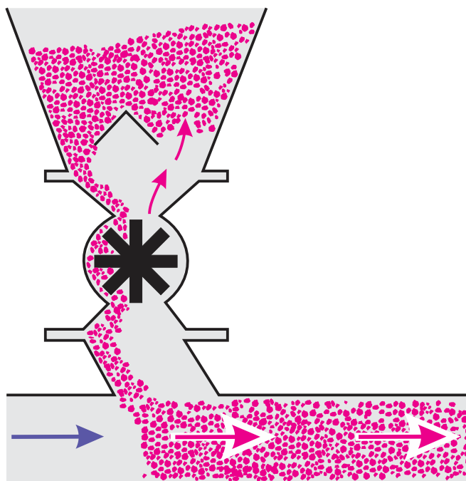
Figure 6.27. Illustration of a rotary airlock feeding a pneumatic conveying line.
