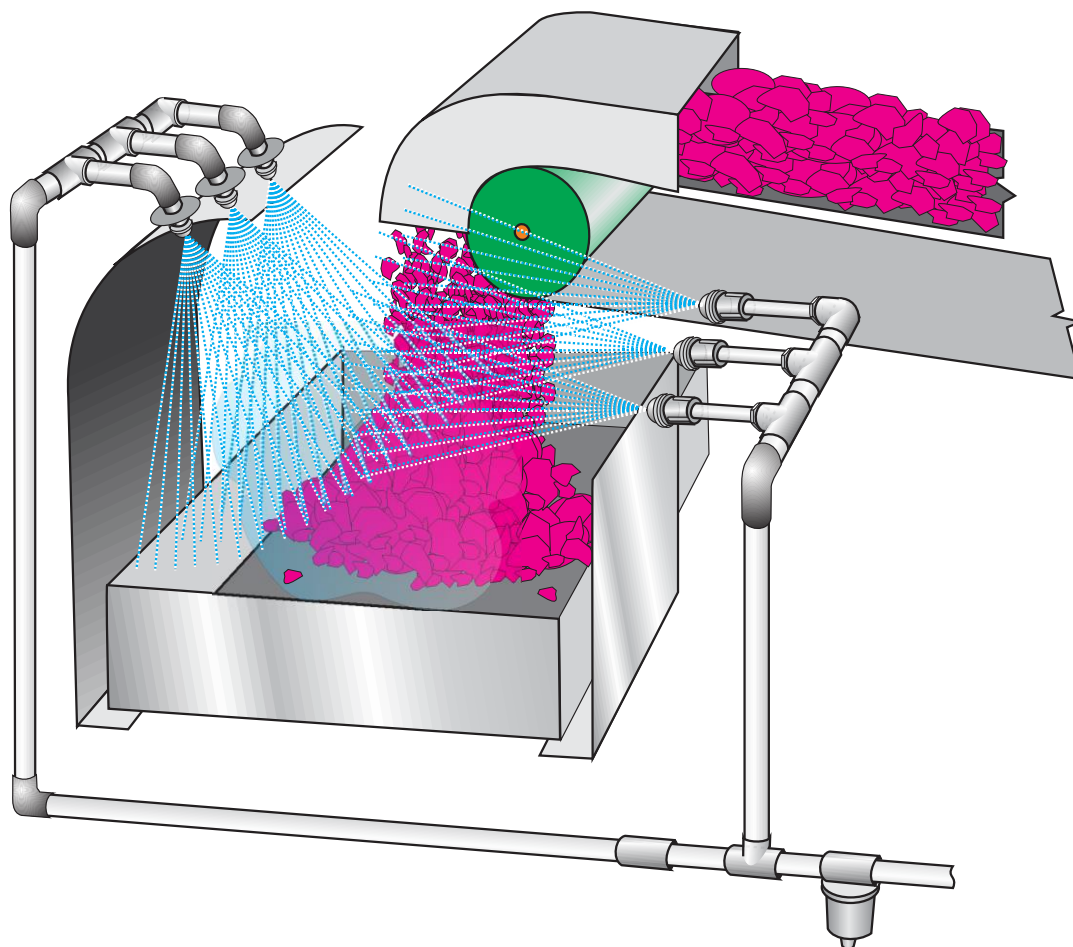
Figure 3.2. Common dust control application illustrating nozzle positioning.
