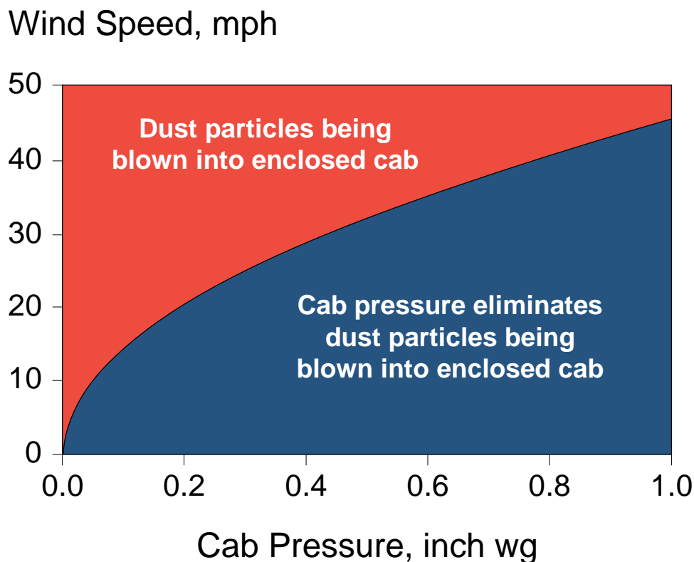
Figure 10.7. Graph showing how positive cab pressure is necessary to prevent dust-laden air from infiltrating an enclosed cab at various wind velocities.
