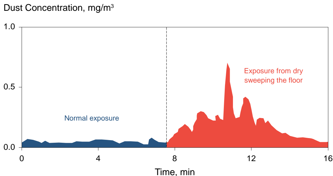
Figure 9.15. Graph showing an increase in a coworker's dust exposure one floor up from floor sweeping.
