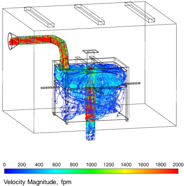
Figure 4.10. The pathline of bailing airflow colored by a velocity magnitude of 0 to 2,000 feet per minute (fpm) with a 6-inch-wide shelf.
