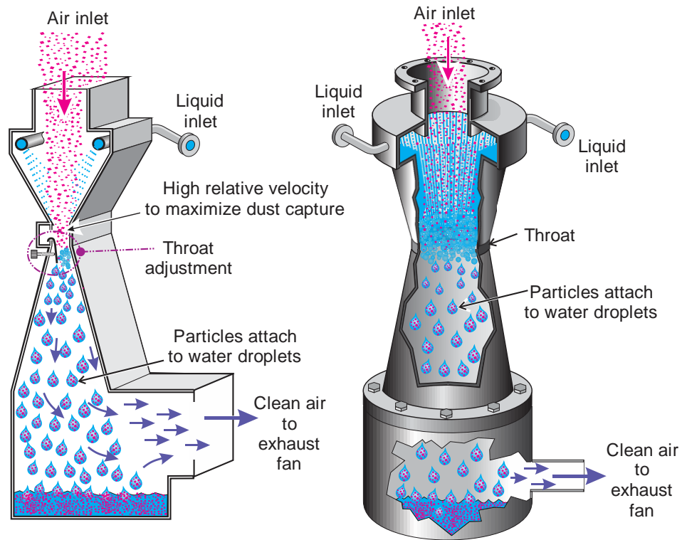
Figure 2.23. Illustration of typical designs for a venturi scrubber.
