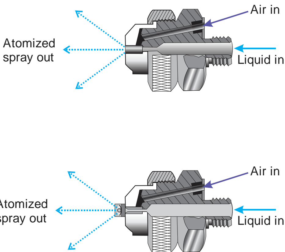
Figure 3.5. Two styles of air atomizing nozzles. The top illustration shows a typical internal mix nozzle. The bottom illustration shows a typical external mix nozzle [adapted from SSCO 2018].
