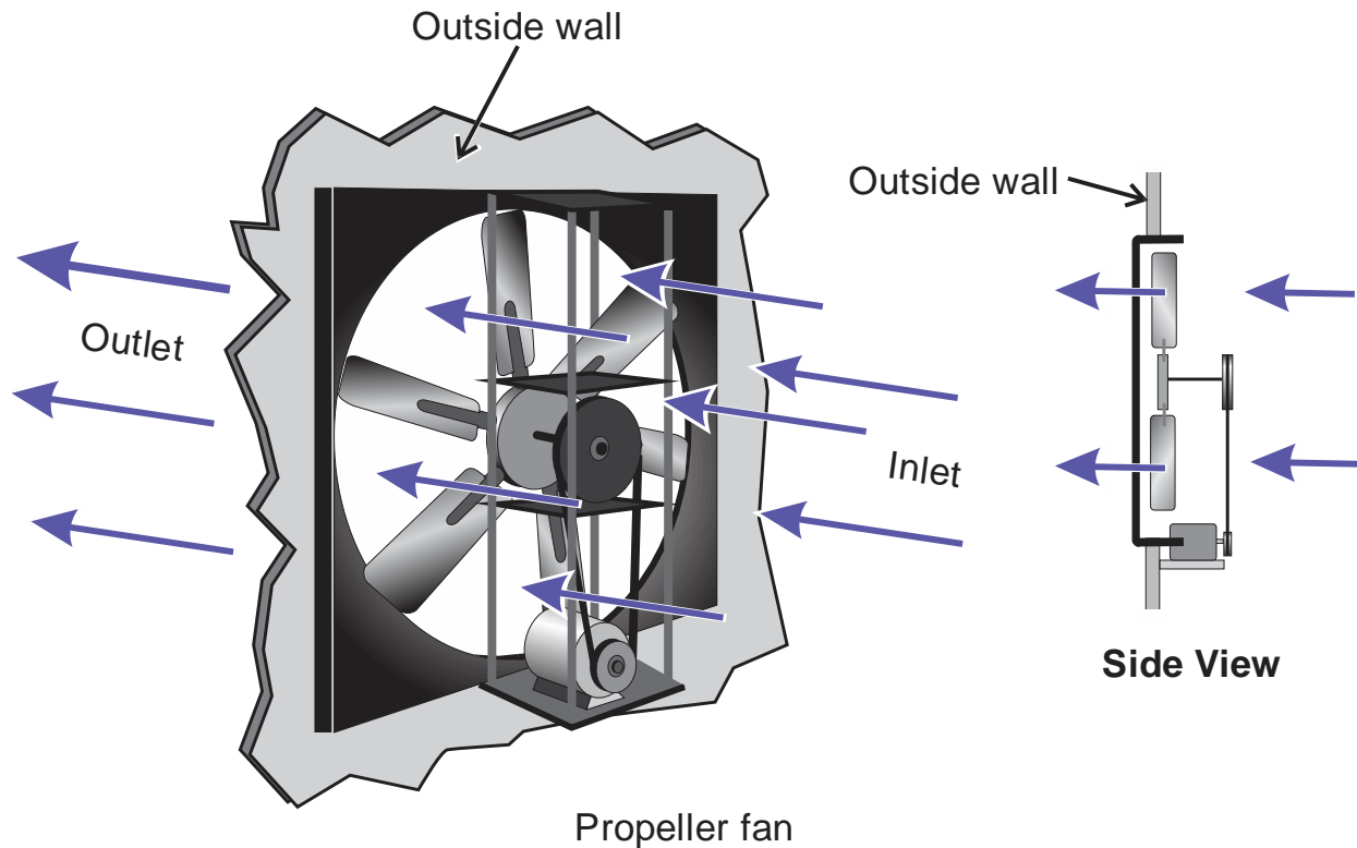
Figure 2.29. Illustration of a wall-mounted propeller fan.
