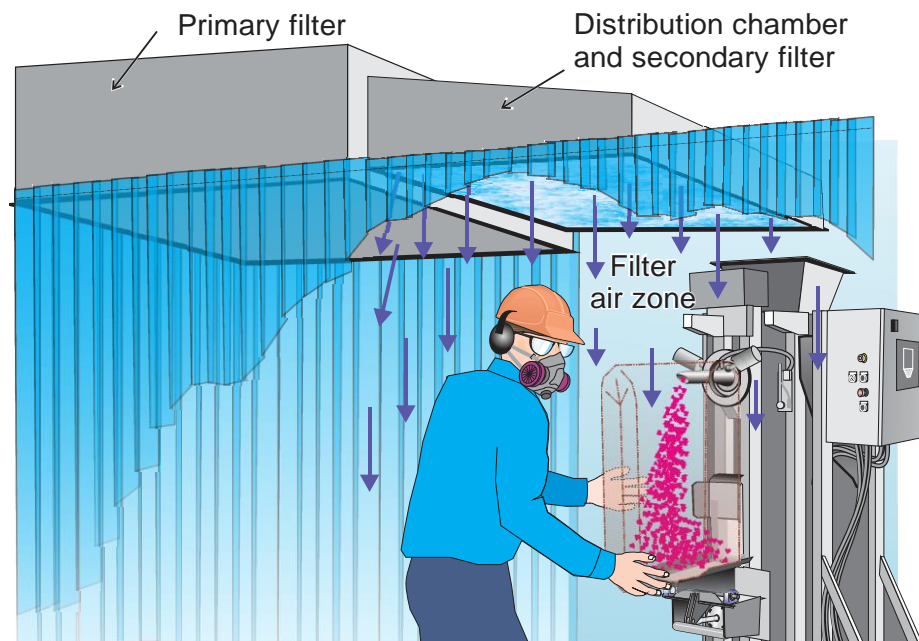
Figure 7.12. Illustration of an Overhead Air Supply Island System (OASIS) positioned over a bag operator to deliver clean filtered air down over the work area.
