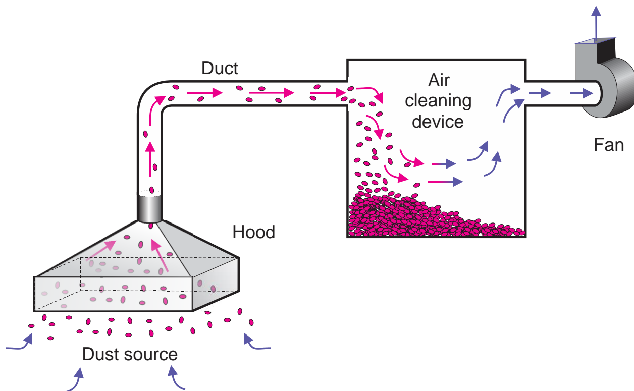
Figure 2.2. Basic illustration of a simple exhaust system with the major components of the hood, duct, air cleaning device, and fan.
