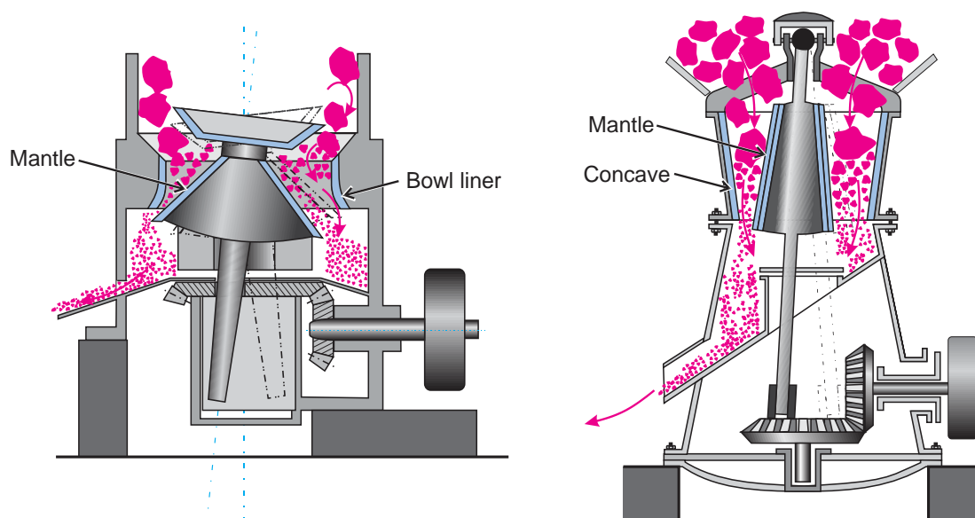
Figure 5.2. Illustrations of two examples of compressive crushers. The left illustration shows a cone crusher with material being crushed between the cone mantle and bowl liner. The right illustration shows a gyratory crusher with material being crushed between the gyratory head and the frame concave.
