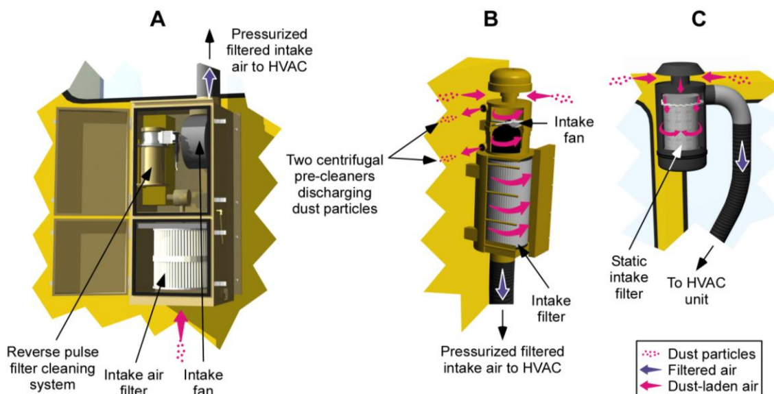
Figure 10.8. Illustration of two types of recommended powered intake systems. A and B show a powered unit design (recommended) while C shows a static, non-powered system (not recommended).
