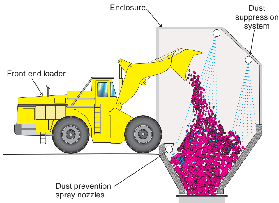
Figure 3.16. Illustration of a typical loader dump dust control application.
