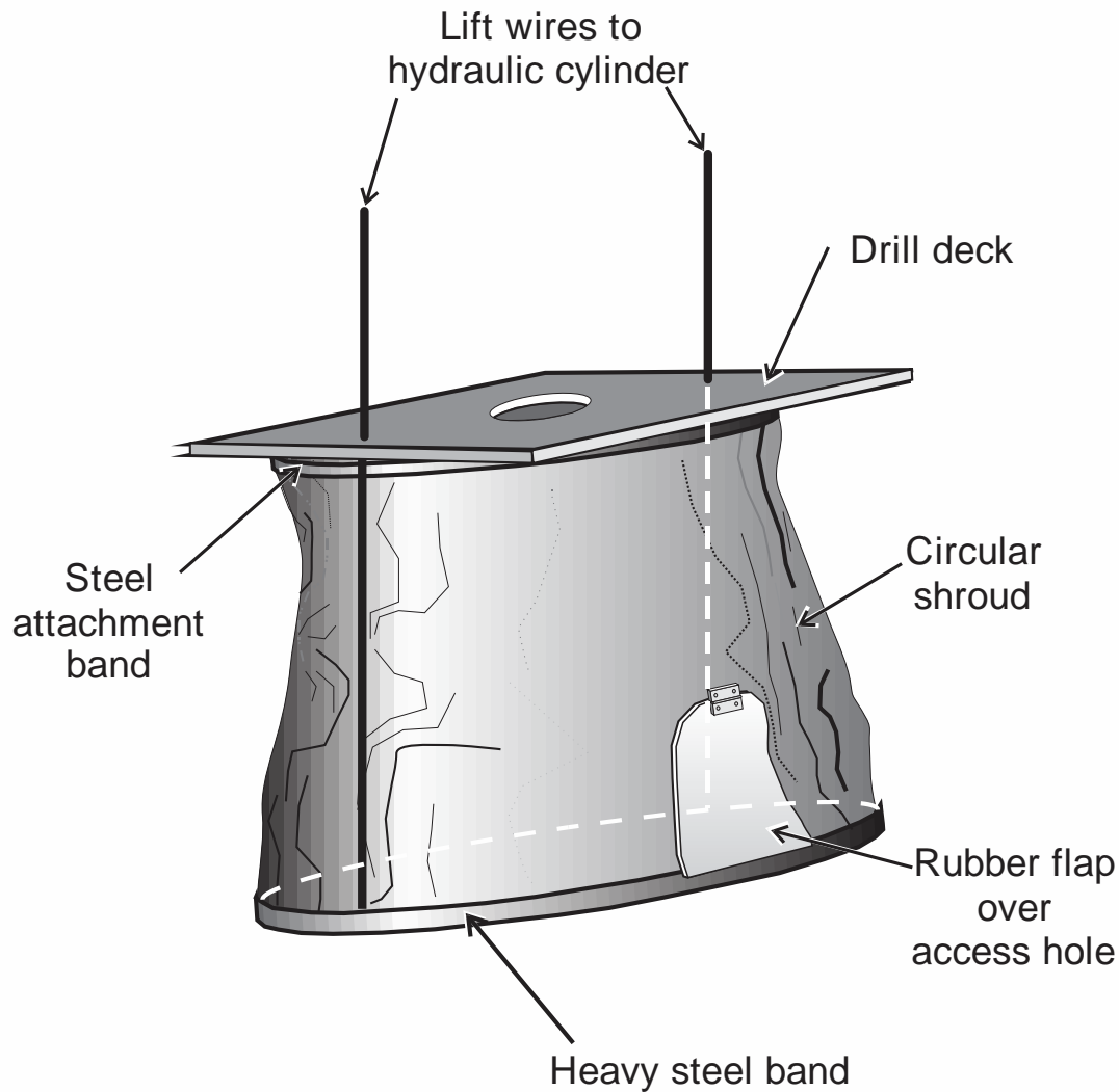
Figure 4.6. Illustration of a circular shroud design.
