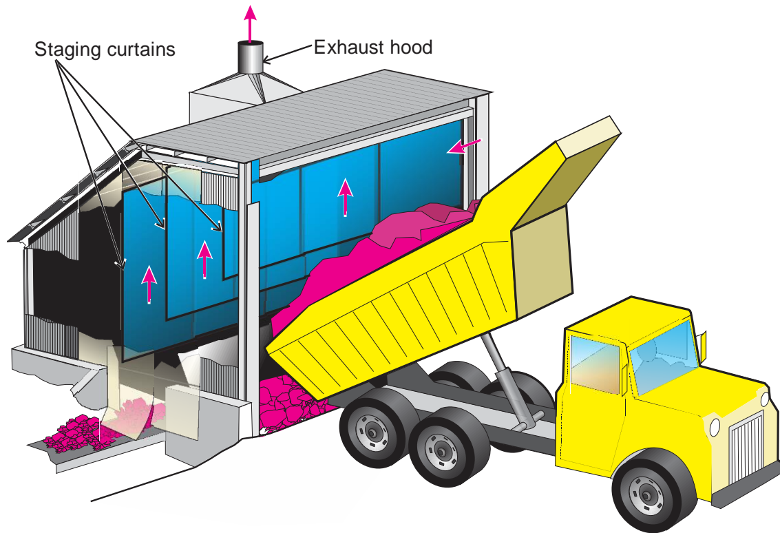
Figure 5.5. Illustration of a dry (exhaust) dust control system with a partial enclosure at a crusher dump loading operation.
