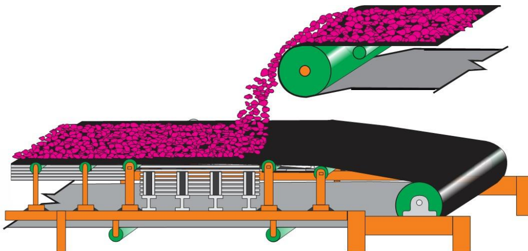
Figure 6.8. Basic illustration of material transfer from a top conveyor to a bottom conveyor.
