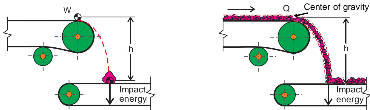
Figure 6.5. Calculations for determining material impact loading at a conveyor transfer point [adapted CEMA Standard 575–2013], with illustrations depicting the impact from a single lump (left) and a homogenous stream (right).
