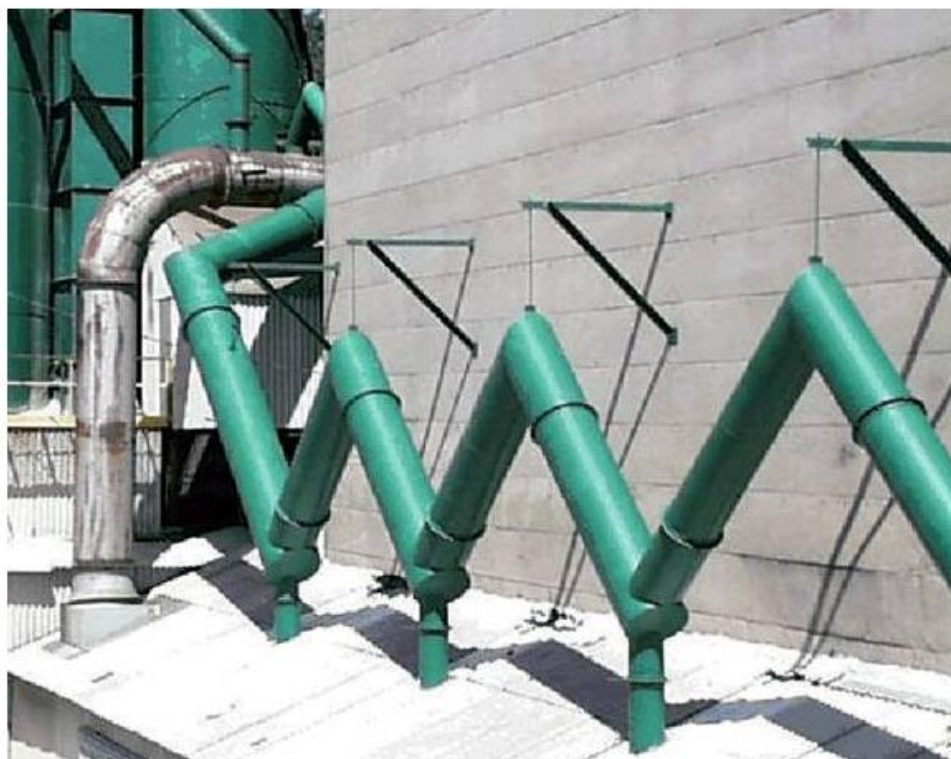
Figure 2.11. Sawtooth (“grasshopper”) design of a low-velocity system with a drop-out duct back into the process at the base of each leg.
