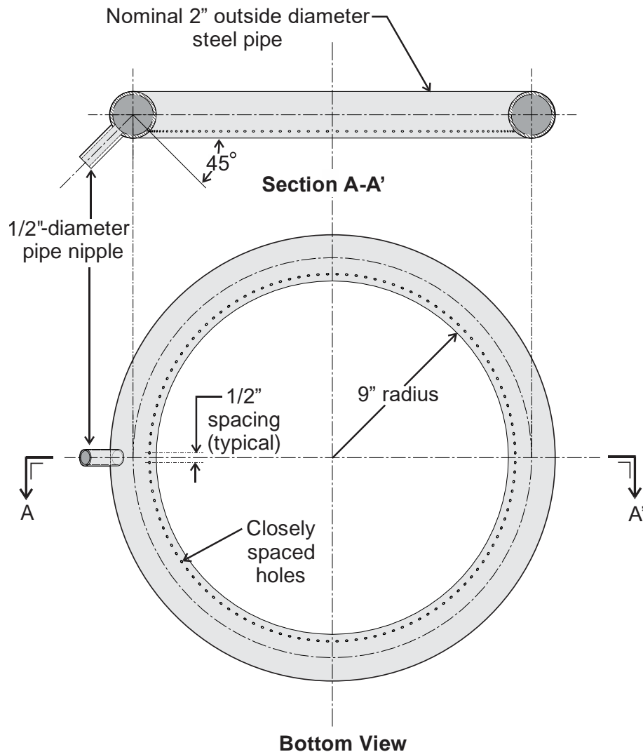
Figure 4.17. Air ring seal used to impede the movement of dust particles through an opening.
