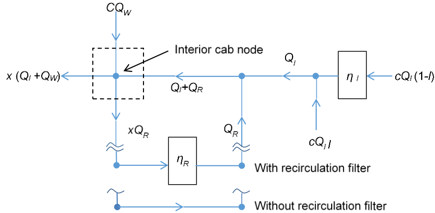
Figure 10.2. Two- and one-filter cab systems with and without a recirculation filter. Q's denote air quantities, x's & c's denote contaminant concentrations, and η's denote filter efficiencies.
