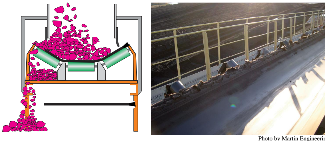
Figure 6.7. Material being improperly fed onto a conveyor belt. The left illustration shows how improper loading can move the belt into the structure with the consequence of damage to the belt and support structure. The right photo shows the resulting belt damage that can occur from long-term belt structure contact.
