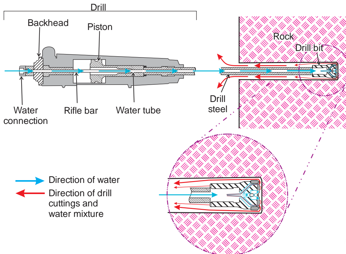
Figure 4.20. Illustration of water flow during a drilling operation to demonstrate water flushing of the drill cuttings. The water flows through the drill into the center of the drill steel and out the end of the drill bit to remove the cuttings from the drill hole.
