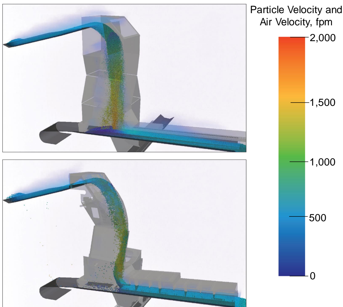
Figure 6.13. Simulation of engineered flow chute, with particle velocity and air velocity represented. The top image shows the original design in which the material was escaping from the hood. The bottom image shows the modified design resulting in improved flow of air and material.
