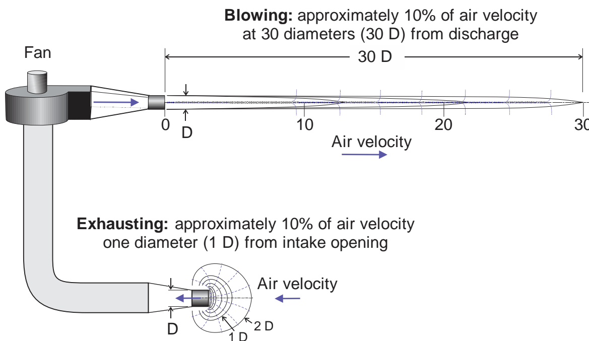
Figure 2.3. Illustration comparing the ventilation characteristics for a blowing versus an exhausting system [adapted from Hartman et al. 1997].
