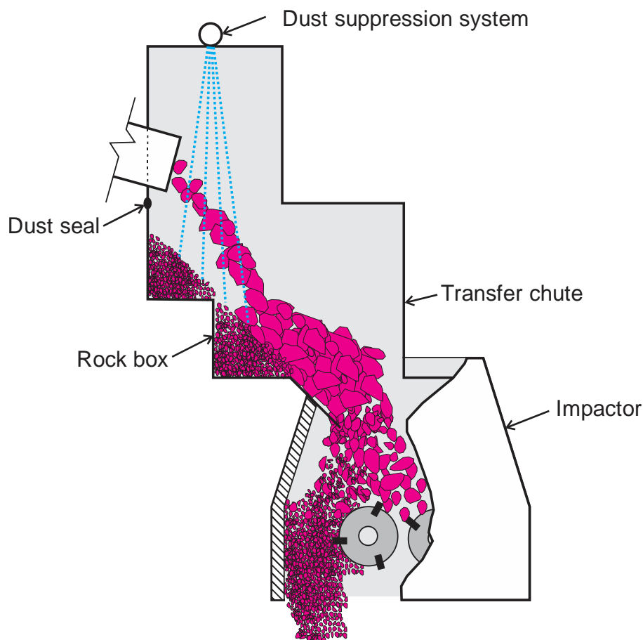
Figure 5.10. Illustration of a wet dust control approach with a transfer chute/rock box enclosure at a crusher loading operation.
