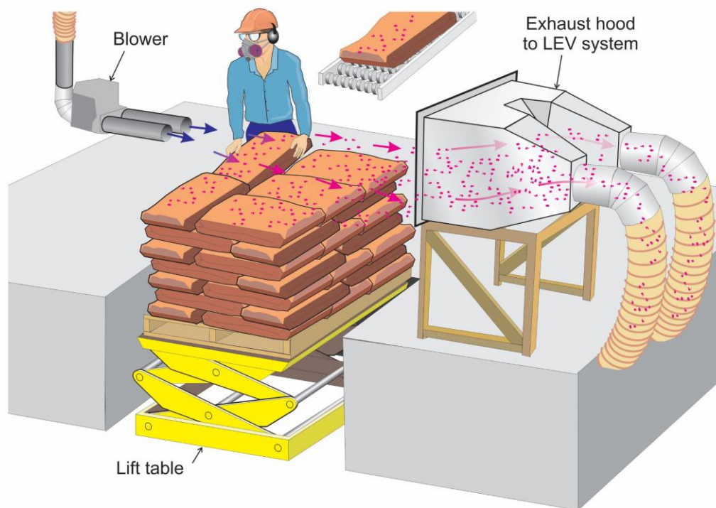
Figure 7.17. Illustration of a semi-automated bag palletizing system. This system provides ergonomic improvements to the bag stacking process with a push-pull ventilation system used to capture the dust generated.
