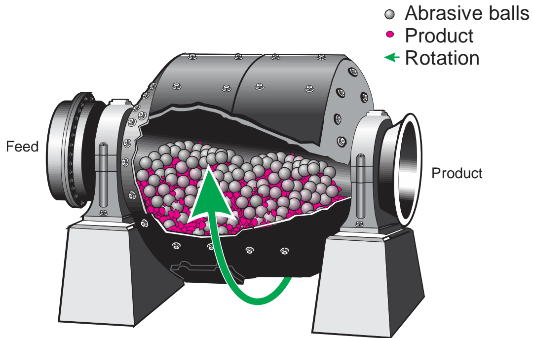
Figure 5.12. Cutaway illustration of a ball mill.
