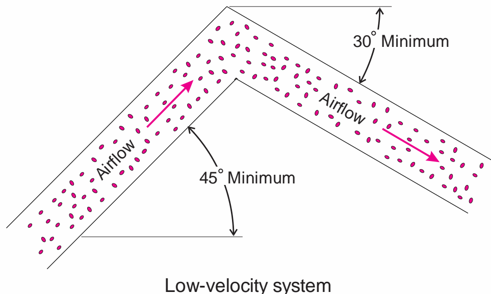
Figure 2.12. Illustration of duct design angles for low-velocity systems.
