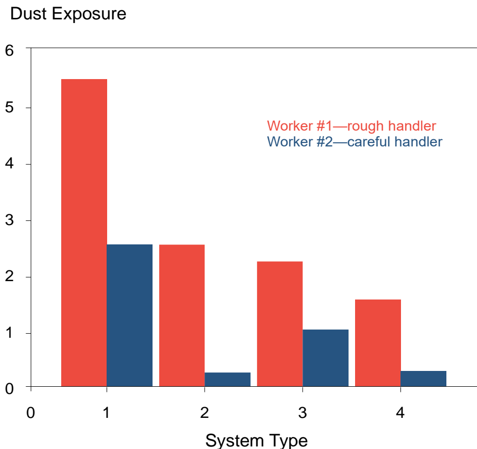
Figure 9.21. Bar chart comparing two workers' respirable dust exposure while performing their jobs with different control techniques being implemented.
