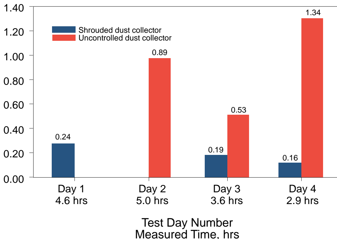
Figure 4.16. Comparison of dust concentrations of uncontrolled dust collector dump to shrouded dust collector dump.
