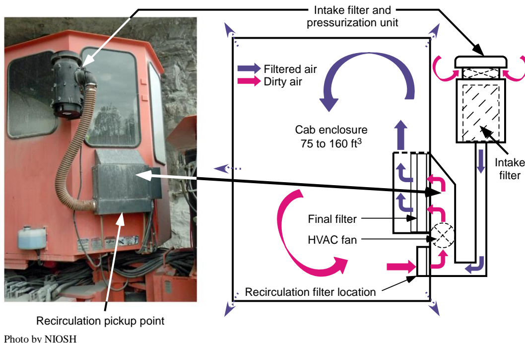
Figure 10.3. Intake, recirculation, and final filter locations within an HVAC system designed by an original equipment manufacturer and field tested by NIOSH.
