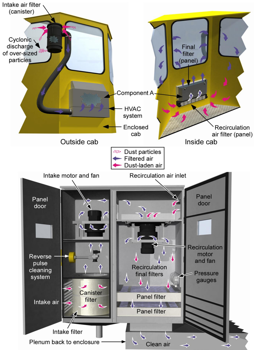
Figure 10.6. Examples of effective filtration and pressurization system designs. The top illustration shows a system for an enclosed cab using a cyclonic precleaning canister intake air filter with a panel recirculation and final filter. The bottom illustration shows a system design for control rooms and operator compartments with a reverse pulse cleaning canister intake filter and two panel filters in series used for recirculation cleaning and final filter design.
