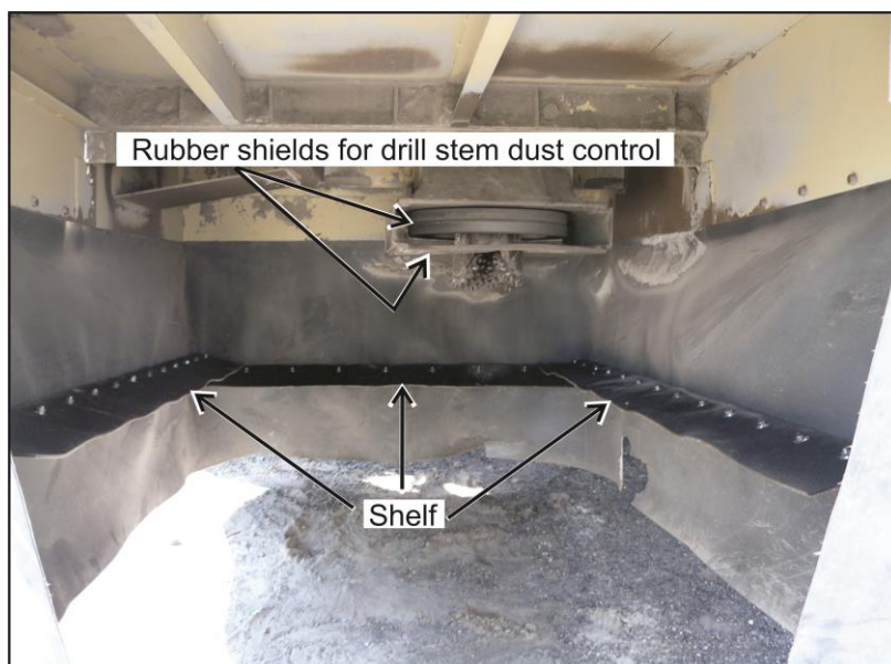
Figure 4.12. Air-blocking shelf installed on the inside perimeter of the drill shroud of a blasthole drill. Note the overlap in the rear corners to eliminate any gaps in the shelf perimeter.
