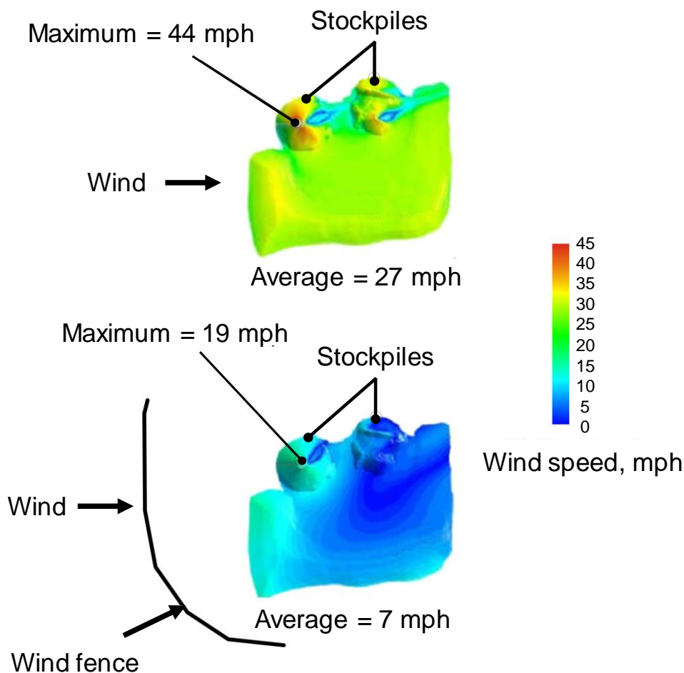
Figure 11.14. Plan view of the area around stockpiles before and after installation of a wind fence as determined from computational fluid dynamics (CFD) modeling. The top model represents the stockpile before wind fence installation and the bottom model represents the stockpile afterwards, with CFD modeling illustrating the changes in wind velocities [adapted from Kibbee 2014].
