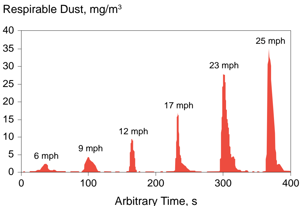
Figure 11.2. Graph showing a dust profile measured at roadside for a haul truck traveling at various speeds (mph) [adapted from Thompson and Visser 2001].
