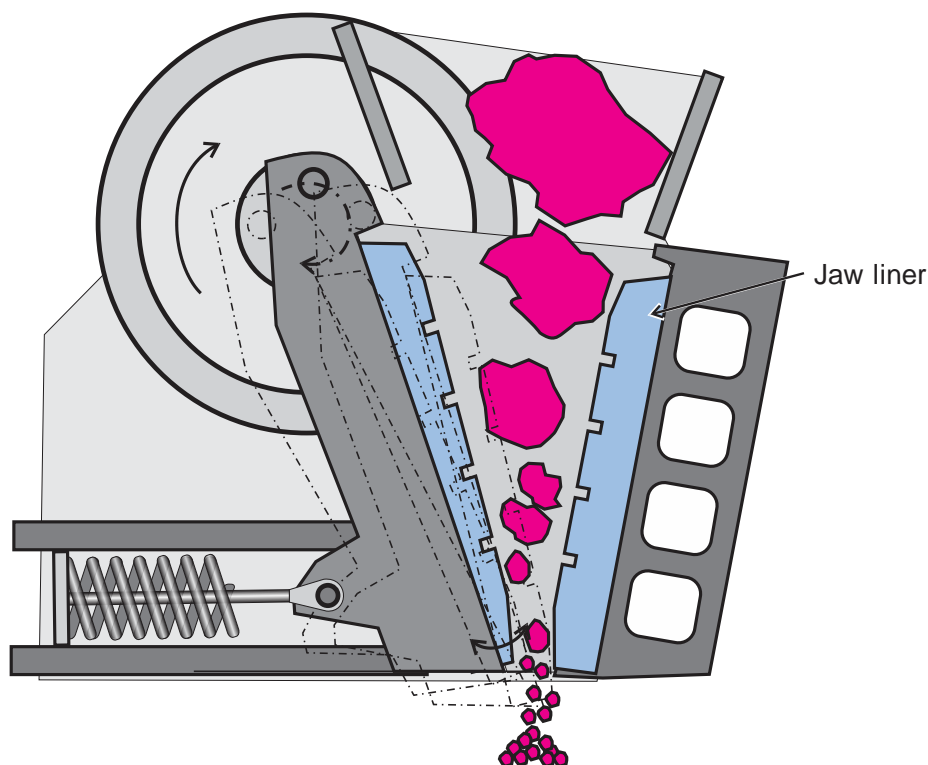
Figure 5.1. Illustration of a jaw crusher showing material being crushed between fixed and reciprocating jaws.
