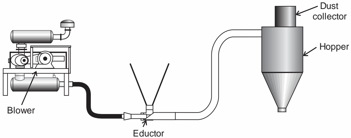
Figure 6.28. Illustration of a conveyance system utilizing a venturi eductor device.
