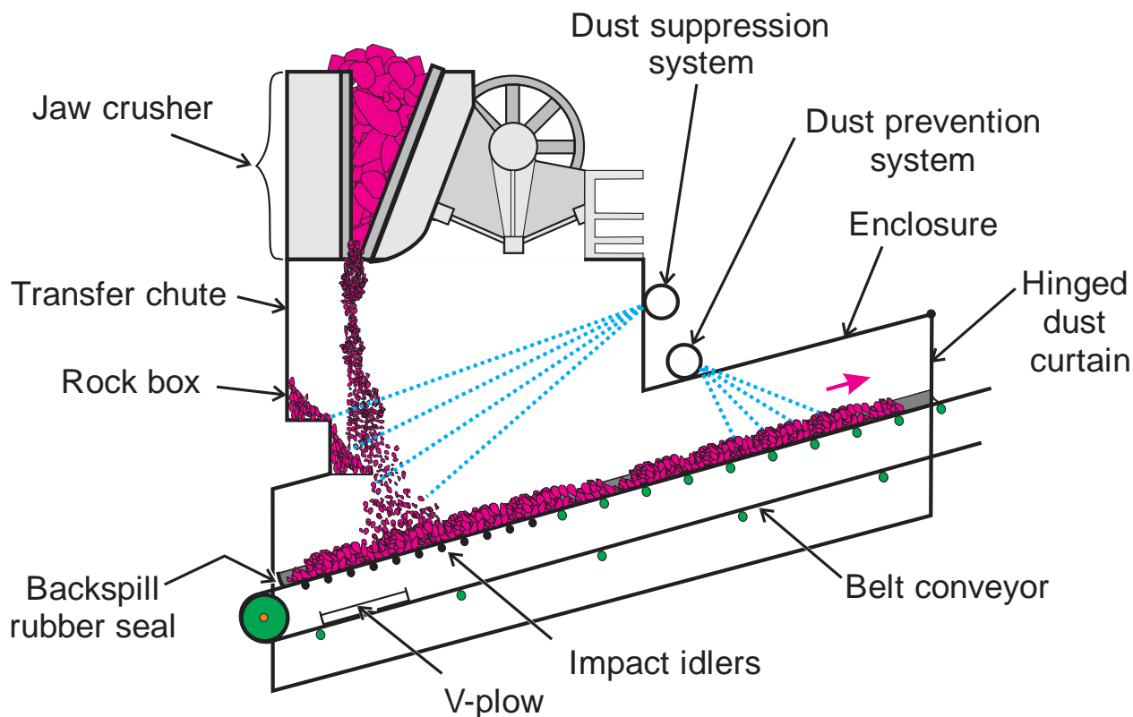
Figure 5.11. Illustration of a wet dust control approach on a crusher discharge/belt loading operation.
