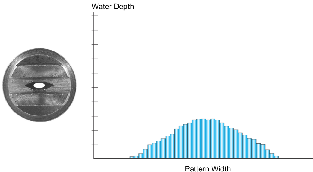
Figure 3.28. Good spray tip showing pattern and distribution graph. Bar height indicates distribution of water over pattern width and shows relatively uniform flow over the width of the pattern [adapted from SSCO 2013].
