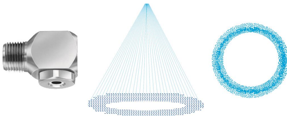
Figure 3.8. Typical hollow cone whirl chamber nozzle and spray pattern. A right angle design is shown [adapted from Schick 2008].
