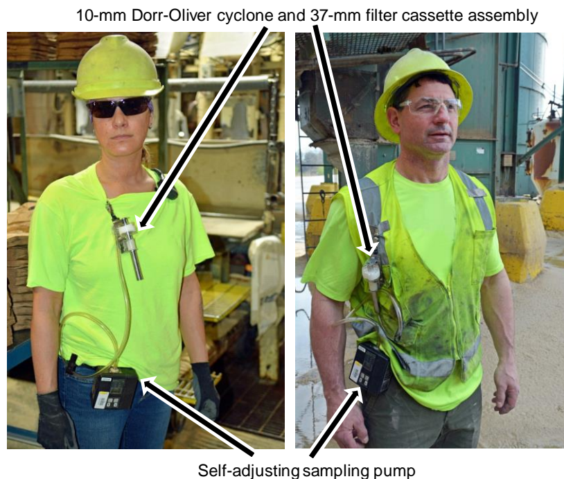
Figure 1.3. Two workers wearing personal gravimetric sampling assemblies. The pump connects to the cyclone/filter unit via Tygon tubing. In these examples, note that the cyclone unit for the worker on the right should be raised to ensure that it is closer to his breathing zone, as it is for the worker on the left.
