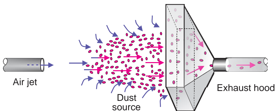
Figure 2.4. Illustration of a simple design of a basic push-pull ventilation system.
