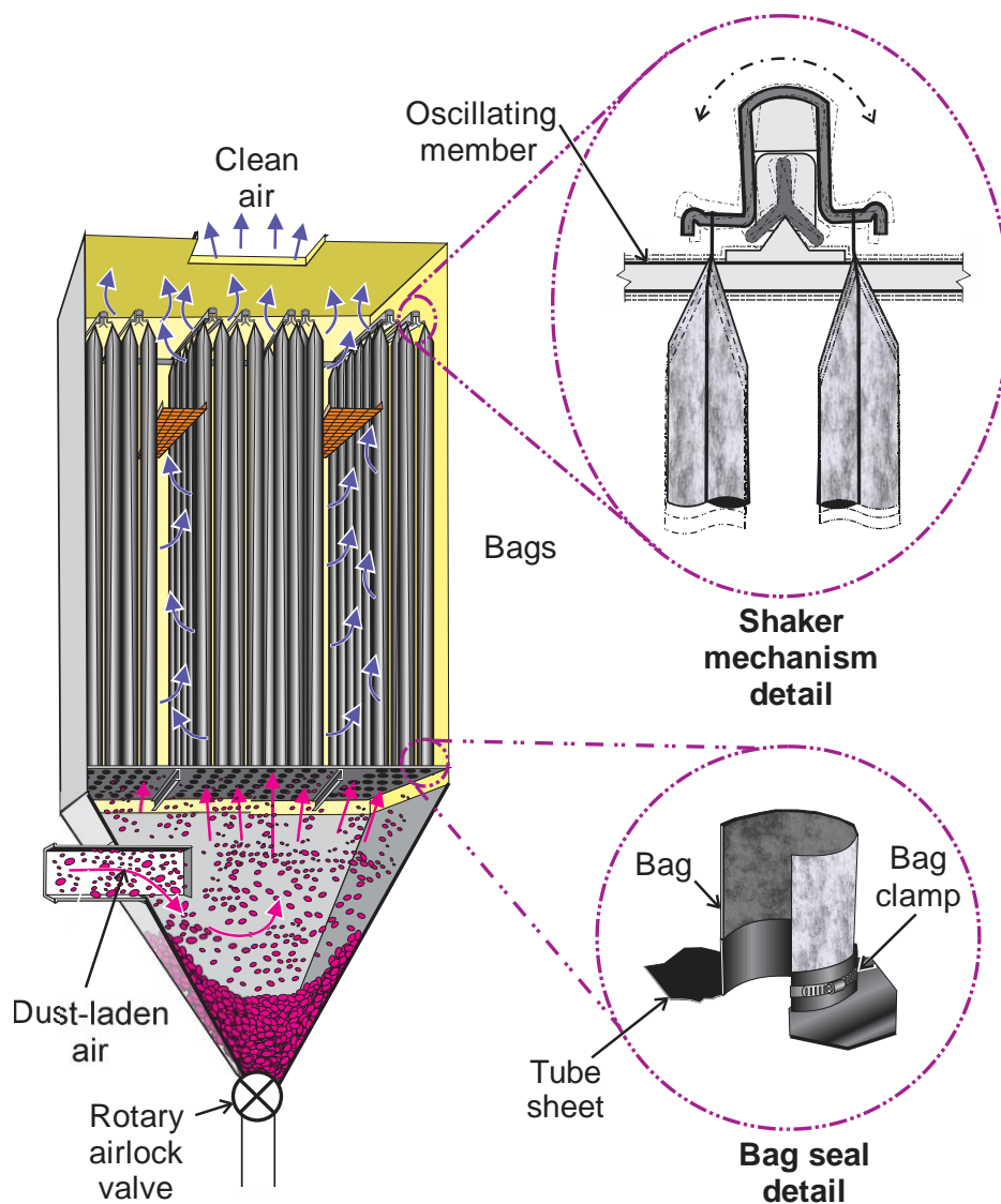
Figure 2.18. Illustration with cutaways showing a typical design of a mechanical shaker dust collector.
