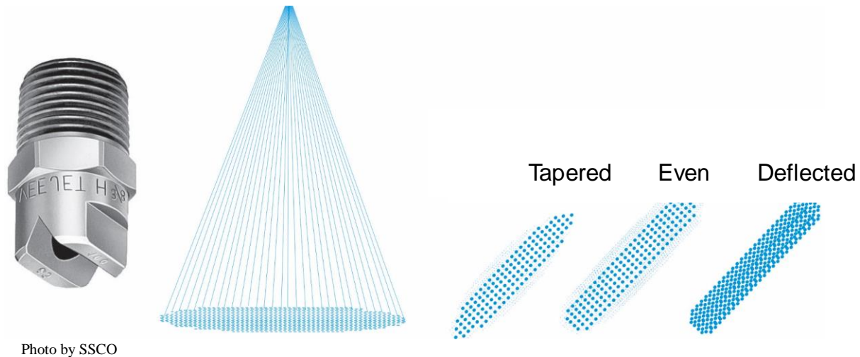
Figure 3.10. Typical flat fan nozzle and spray patterns [adapted from Schick 2008].
