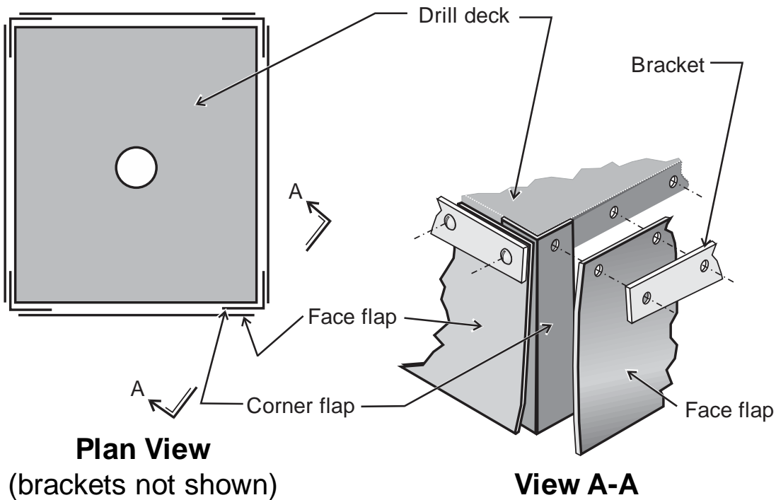
Figure 4.5. Illustration of reinforcing flaps added to each corner of a rectangular deck shroud to reduce leakage.
