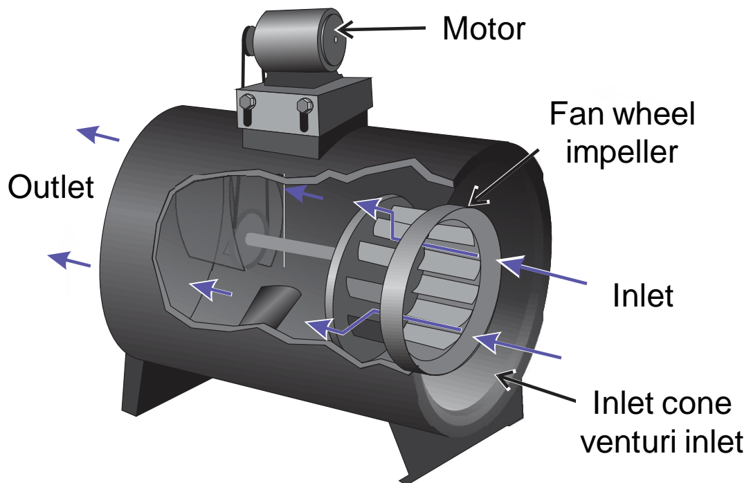
Figure 2.32. Illustration of an axial centrifugal fan showing airflow [adapted from Bleier 1998].
