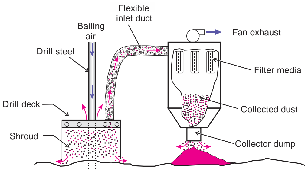
Figure 4.4. Illustration of a basic dry dust collector system on a drill.
