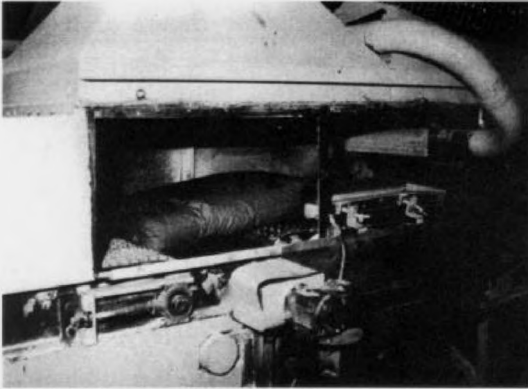
The Bag and Belt Cleaner Device (shown with access panels removed) can handle 50- or 100-lb bags.
