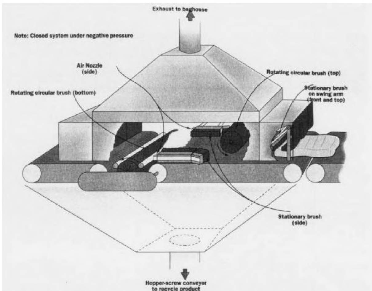
Figure 1: Schematic drawing shows the major components of the Bag and Belt Cleaner Device.
