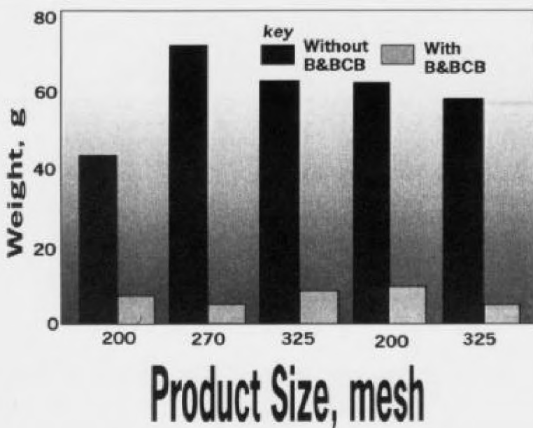
Figure 2: Amount of product removed from the exterior of 50-lb bags by vacuuming, with and without the cleaner device in operation, at evaluation site #2.
